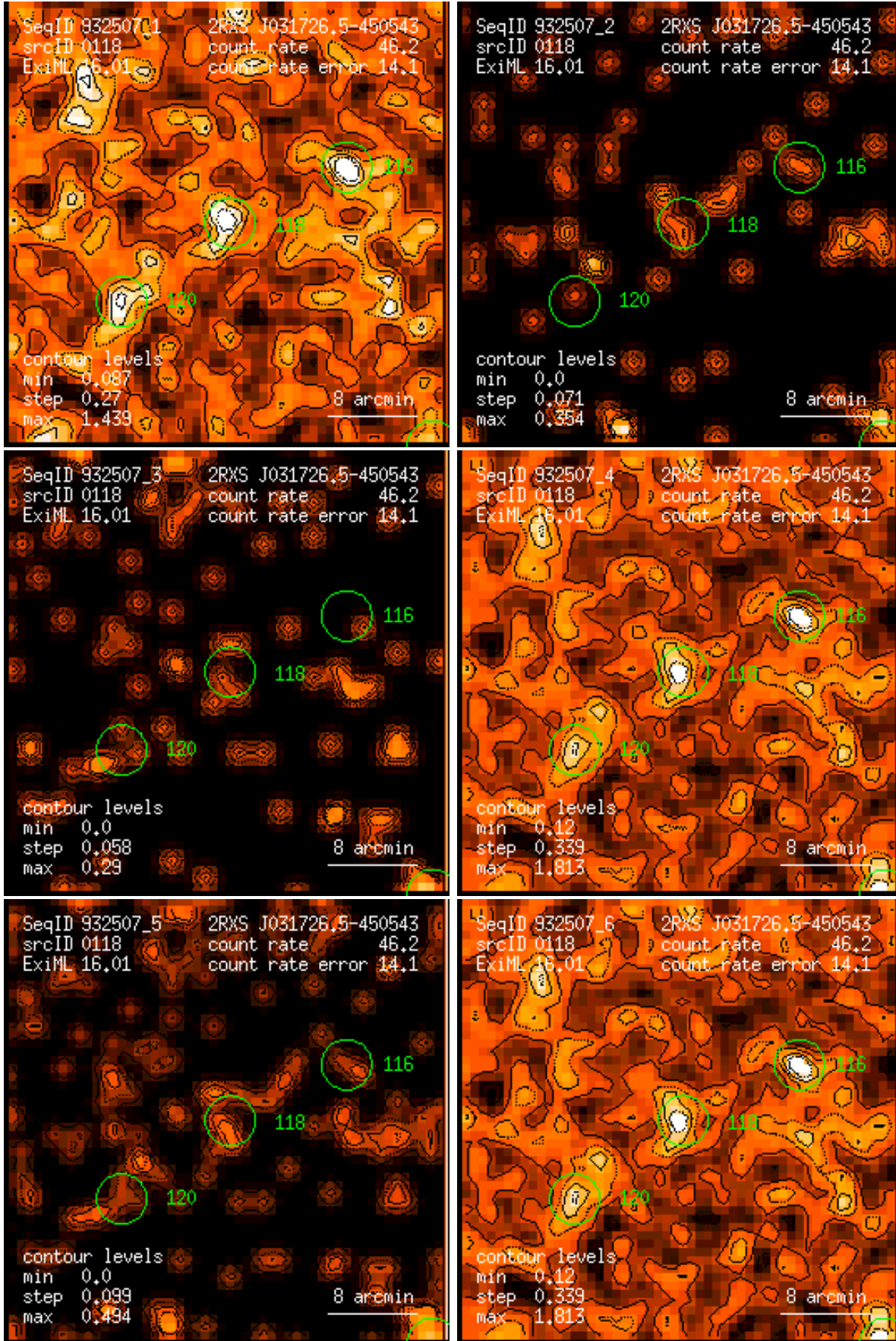
Figure 118: RASS 932507: detection 0118: band rate images, Gaussian filter: (1) PSPC channels 11 – 41, (2) 52 – 90, (3) 91 – 201, (4) 11 – 235, (5) 52 – 201, (6) 11 – 201. Broad band rates in counts/ks. Band rate contour levels in counts/ks/arcmin 2 .
