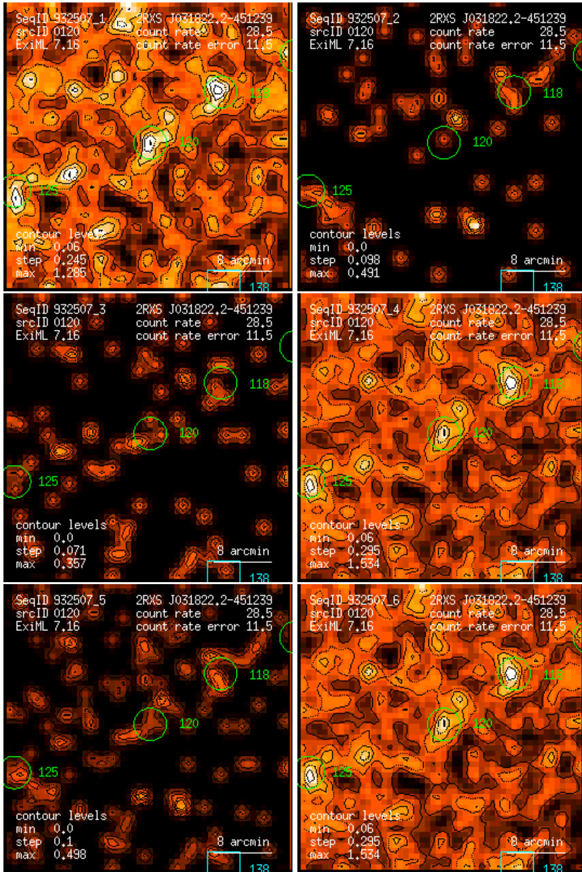
Figure 120: RASS 932507: detection 0120: band rate images, Gaussian filter: (1) PSPC channels 11 – 41, (2) 52 – 90, (3) 91 – 201, (4) 11 – 235, (5) 52 – 201, (6) 11 – 201. Broad band rates in counts/ks. Band rate contour levels in counts/ks/arcmin 2 .
