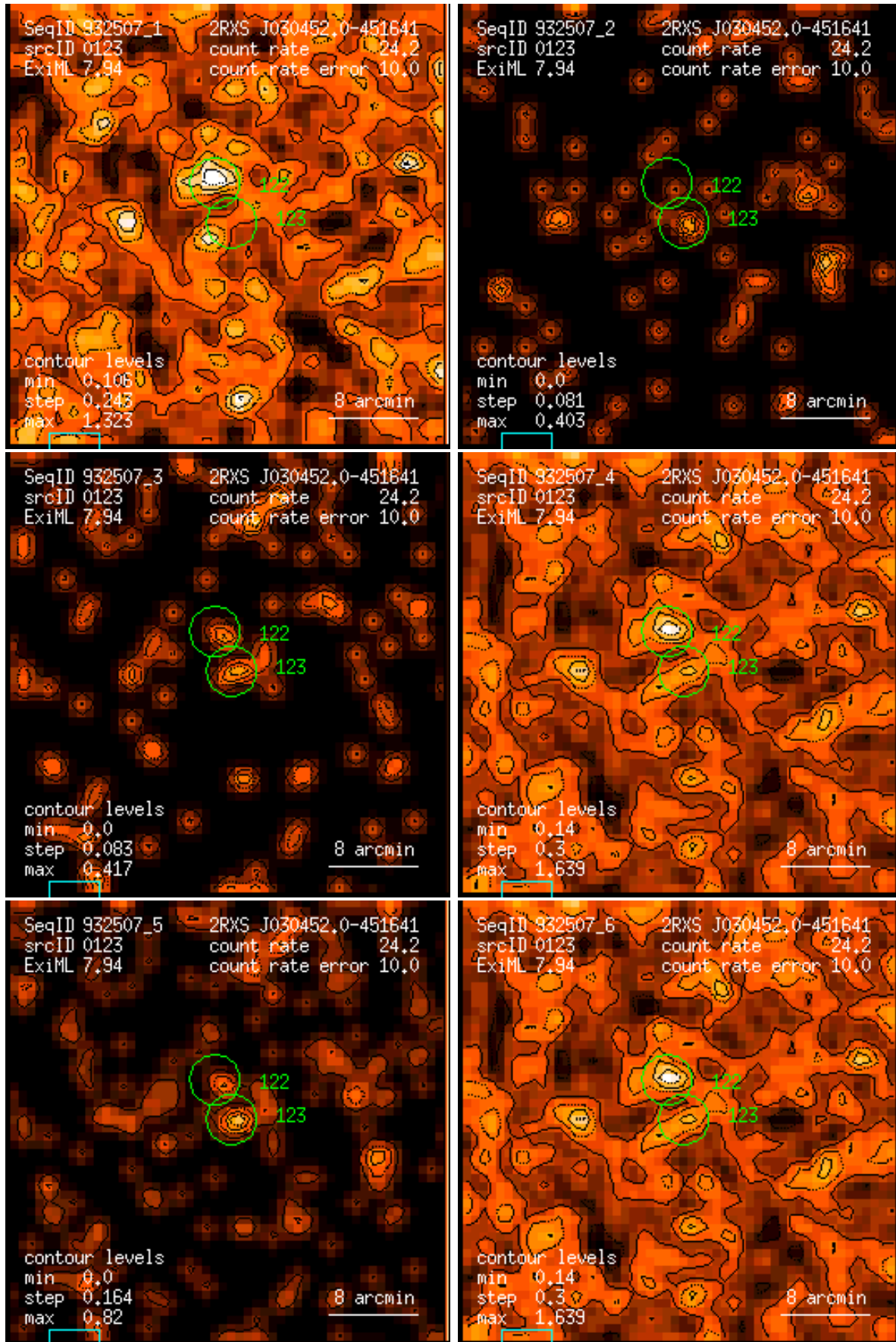
Figure 123: RASS 932507: detection 0123: band rate images, Gaussian filter: (1) PSPC channels 11 – 41, (2) 52 – 90, (3) 91 – 201, (4) 11 – 235, (5) 52 – 201, (6) 11 – 201. Broad band rates in counts/ks. Band rate contour levels in counts/ks/arcmin 2 .
