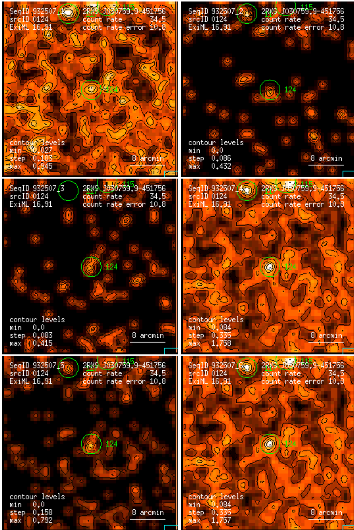
Figure 124: RASS 932507: detection 0124: band rate images, Gaussian filter: (1) PSPC channels 11 – 41, (2) 52 – 90, (3) 91 – 201, (4) 11 – 235, (5) 52 – 201, (6) 11 – 201. Broad band rates in counts/ks. Band rate contour levels in counts/ks/arcmin 2 .
