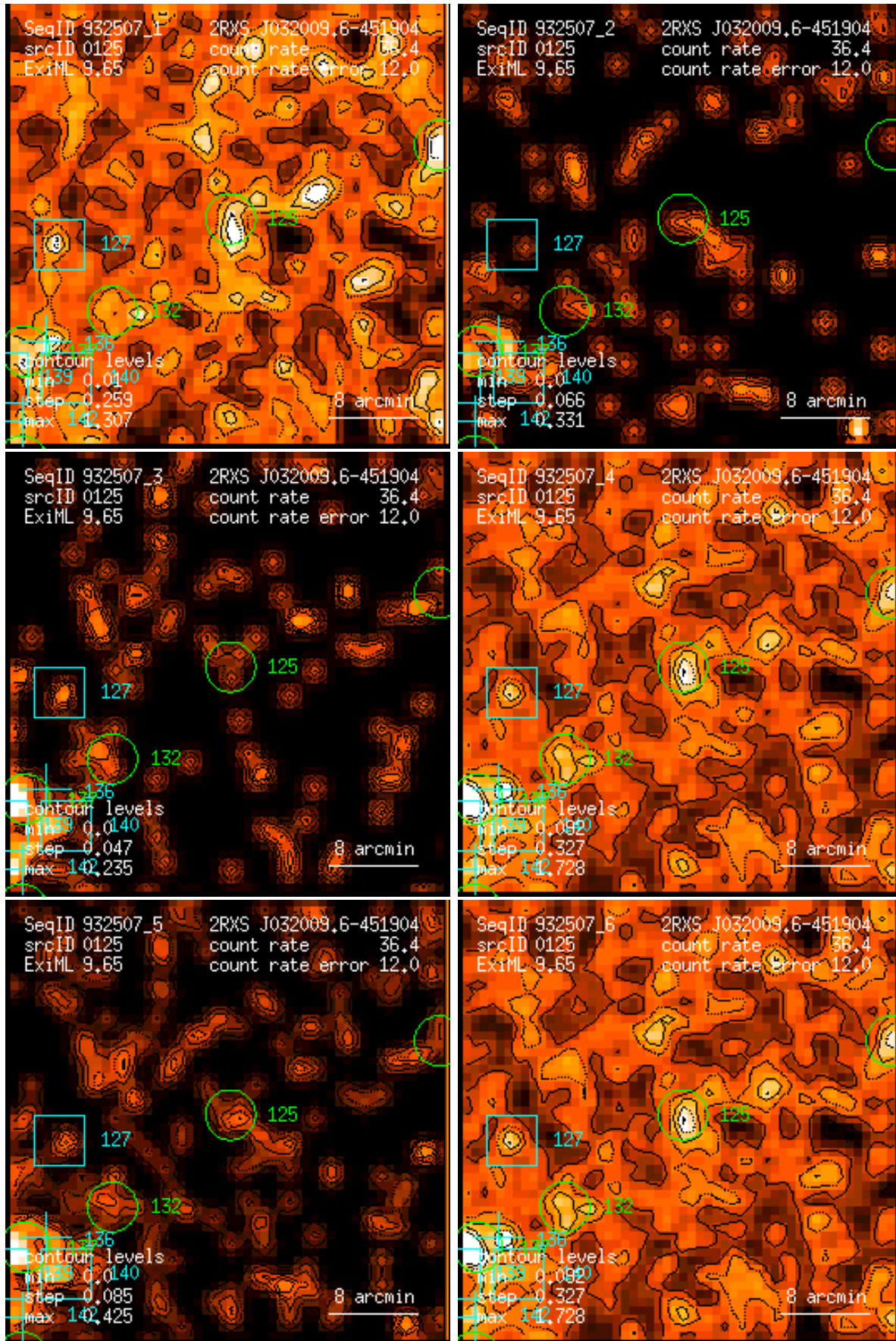
Figure 125: RASS 932507: detection 0125: band rate images, Gaussian filter: (1) PSPC channels 11 – 41, (2) 52 – 90, (3) 91 – 201, (4) 11 – 235, (5) 52 – 201, (6) 11 – 201. Broad band rates in counts/ks. Band rate contour levels in counts/ks/arcmin 2 .
