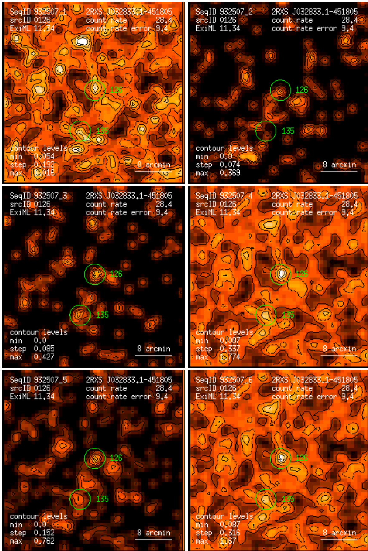
Figure 126: RASS 932507: detection 0126: band rate images, Gaussian filter: (1) PSPC channels 11 – 41, (2) 52 – 90, (3) 91 – 201, (4) 11 – 235, (5) 52 – 201, (6) 11 – 201. Broad band rates in counts/ks. Band rate contour levels in counts/ks/arcmin 2 .
