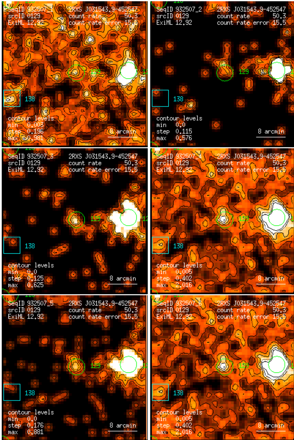
Figure 129: RASS 932507: detection 0129: band rate images, Gaussian filter: (1) PSPC channels 11 – 41, (2) 52 – 90, (3) 91 – 201, (4) 11 – 235, (5) 52 – 201, (6) 11 – 201. Broad band rates in counts/ks. Band rate contour levels in counts/ks/arcmin 2 .
