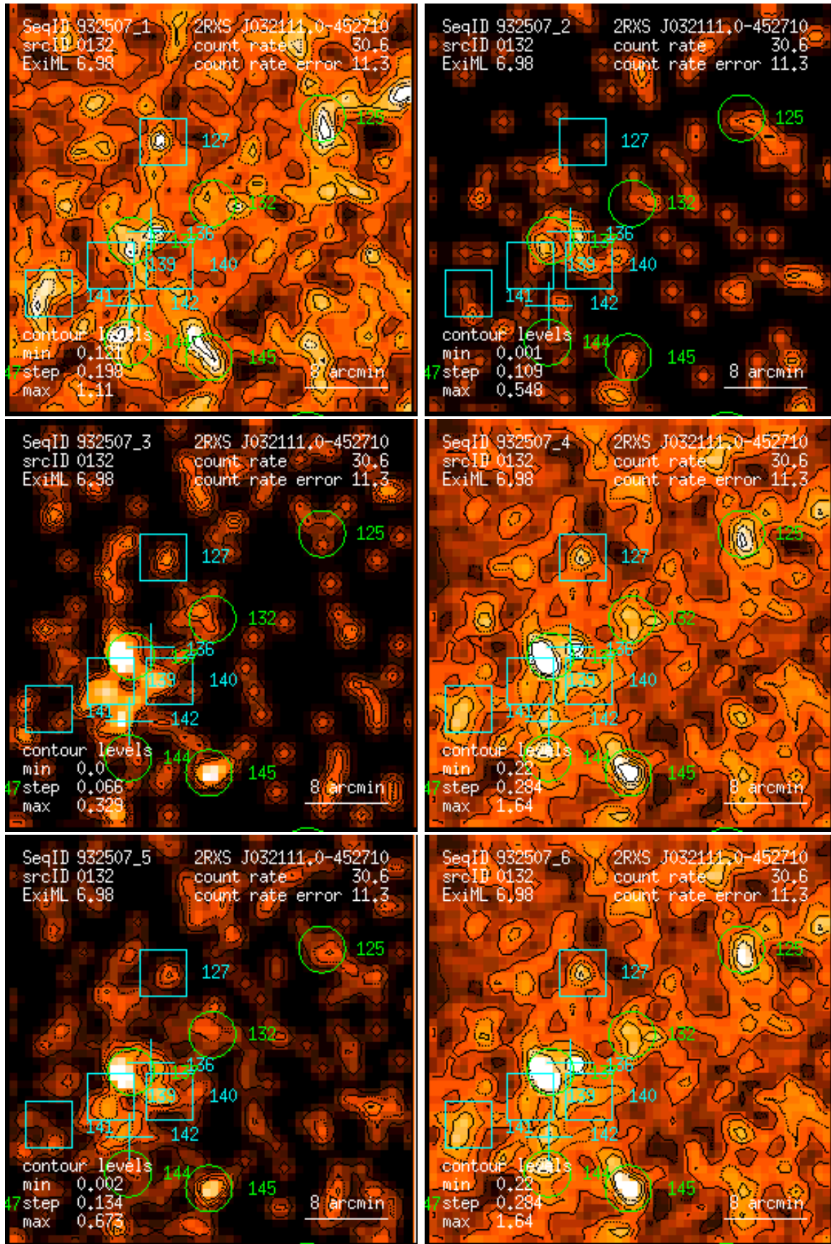
Figure 132: RASS 932507: detection 0132: band rate images, Gaussian filter: (1) PSPC channels 11 – 41, (2) 52 – 90, (3) 91 – 201, (4) 11 – 235, (5) 52 – 201, (6) 11 – 201. Broad band rates in counts/ks. Band rate contour levels in counts/ks/arcmin 2 .
