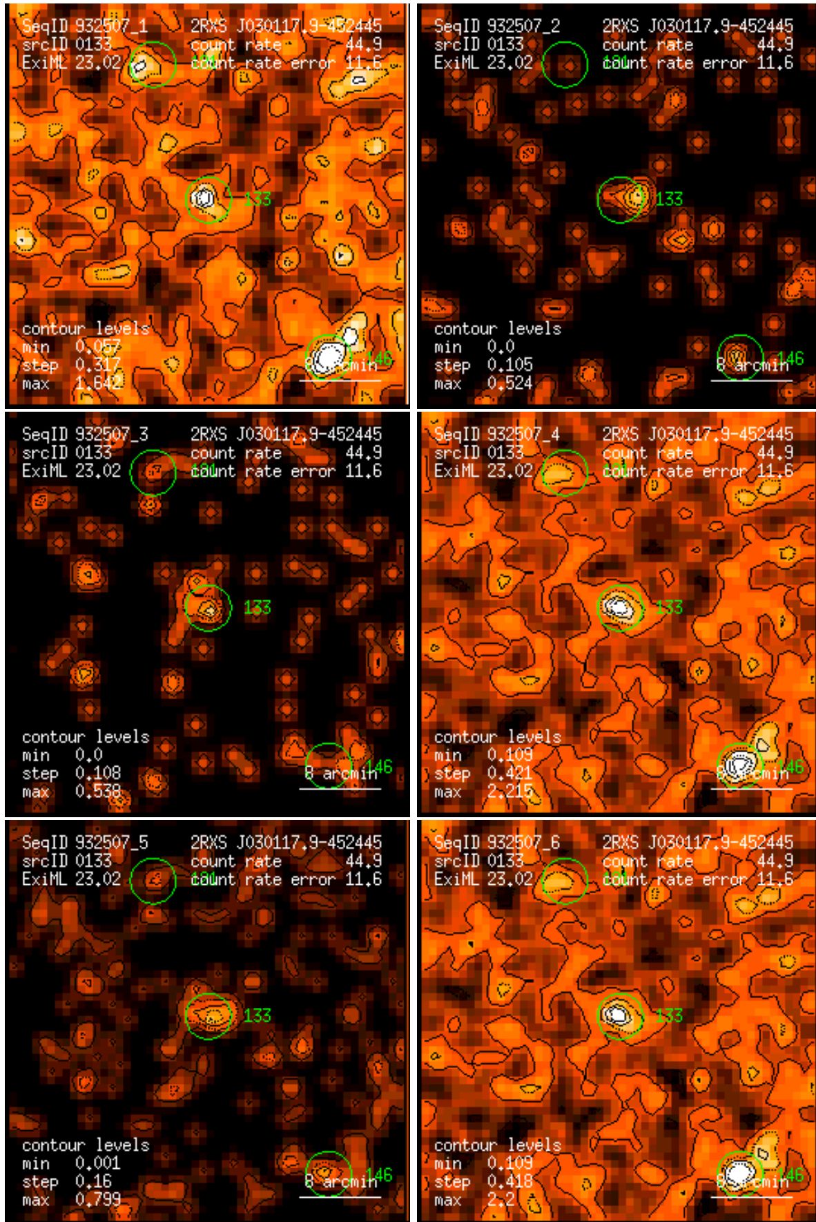
Figure 133: RASS 932507: detection 0133: band rate images, Gaussian filter: (1) PSPC channels 11 – 41, (2) 52 – 90, (3) 91 – 201, (4) 11 – 235, (5) 52 – 201, (6) 11 – 201. Broad band rates in counts/ks. Band rate contour levels in counts/ks/arcmin 2 .
