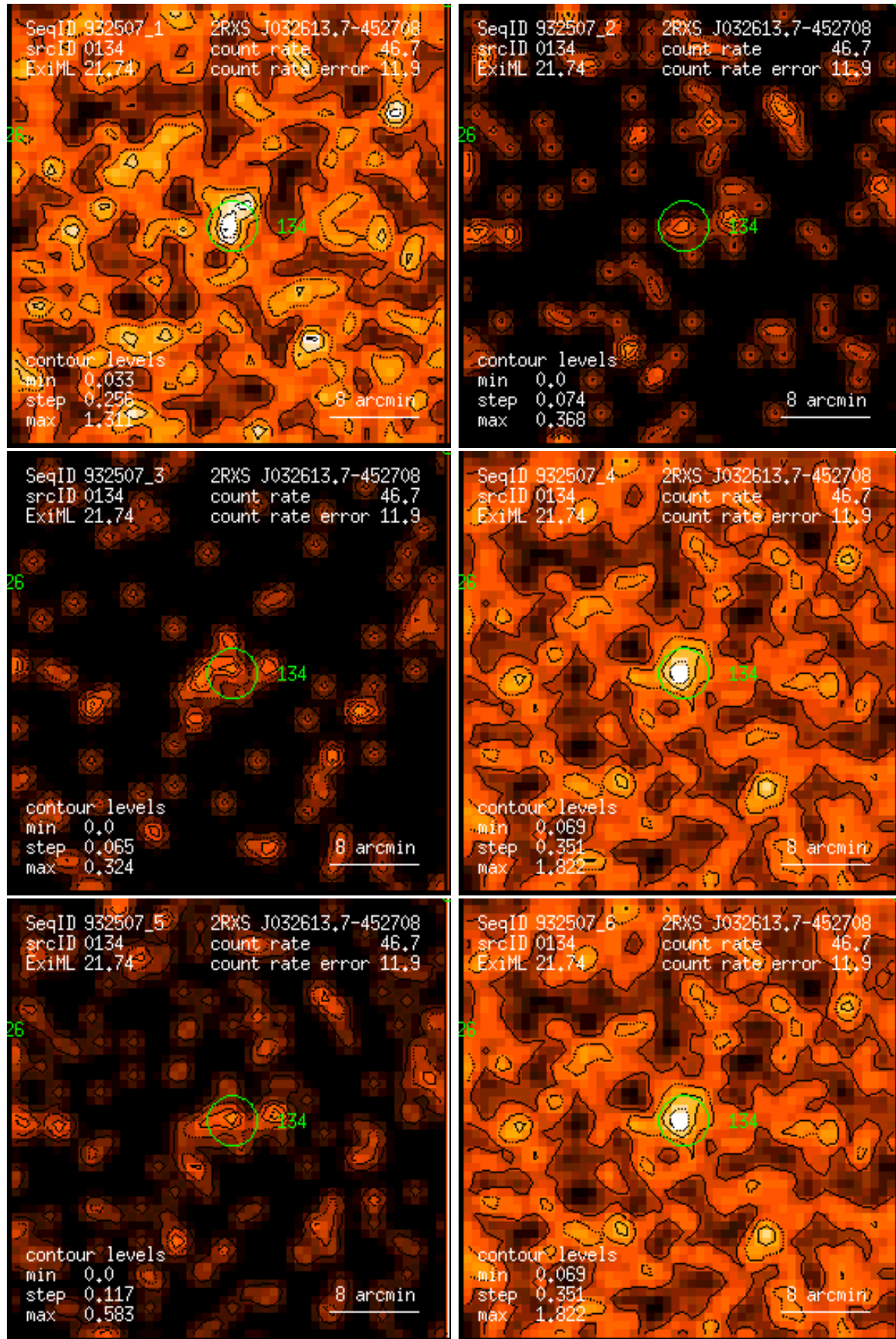
Figure 134: RASS 932507: detection 0134: band rate images, Gaussian filter: (1) PSPC channels 11 – 41, (2) 52 – 90, (3) 91 – 201, (4) 11 – 235, (5) 52 – 201, (6) 11 – 201. Broad band rates in counts/ks. Band rate contour levels in counts/ks/arcmin 2 .
