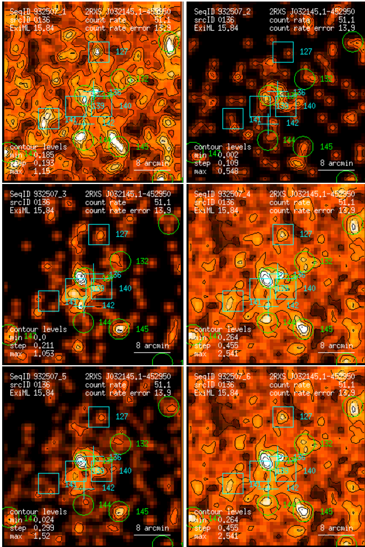
Figure 136: RASS 932507: detection 0136: band rate images, Gaussian filter: (1) PSPC channels 11 – 41, (2) 52 – 90, (3) 91 – 201, (4) 11 – 235, (5) 52 – 201, (6) 11 – 201. Broad band rates in counts/ks. Band rate contour levels in counts/ks/arcmin 2 .
