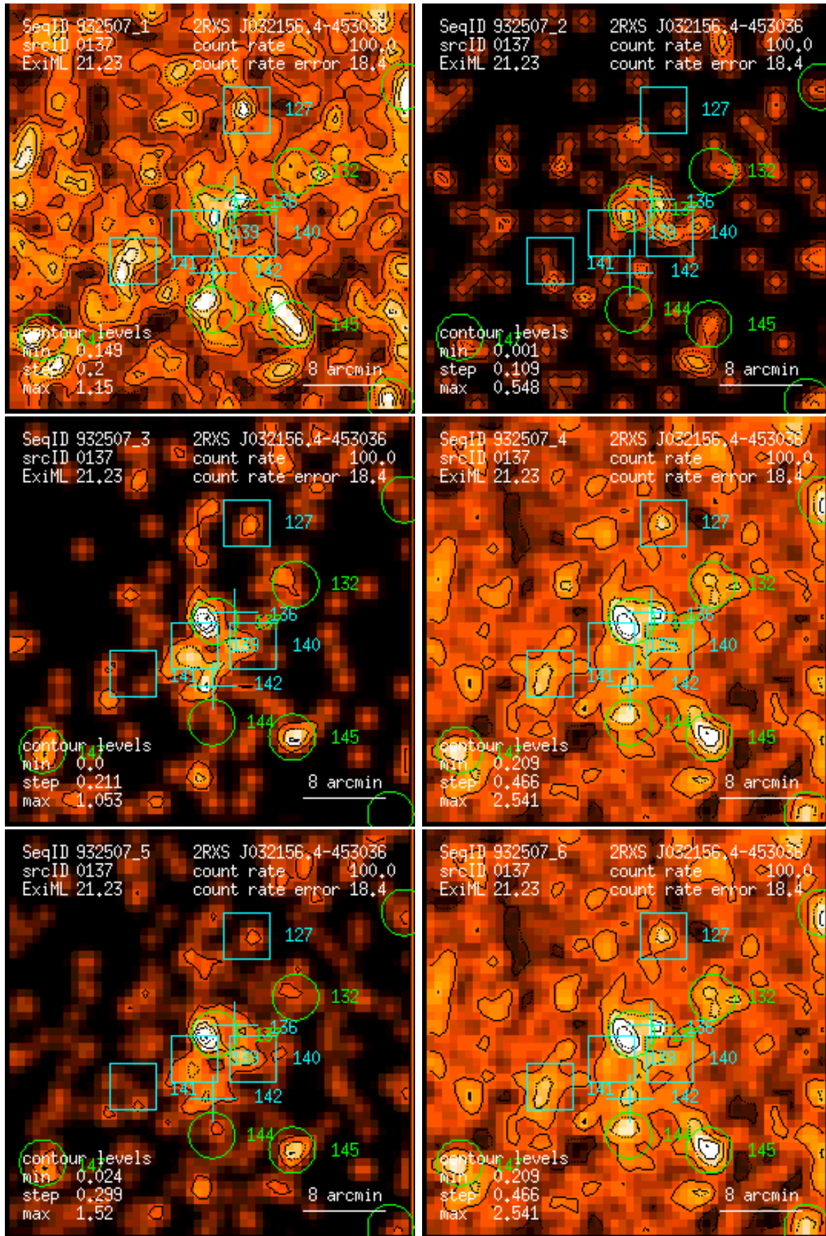
Figure 137: RASS 932507: detection 0137: band rate images, Gaussian filter: (1) PSPC channels 11 – 41, (2) 52 – 90, (3) 91 – 201, (4) 11 – 235, (5) 52 – 201, (6) 11 – 201. Broad band rates in counts/ks. Band rate contour levels in counts/ks/arcmin 2 .
