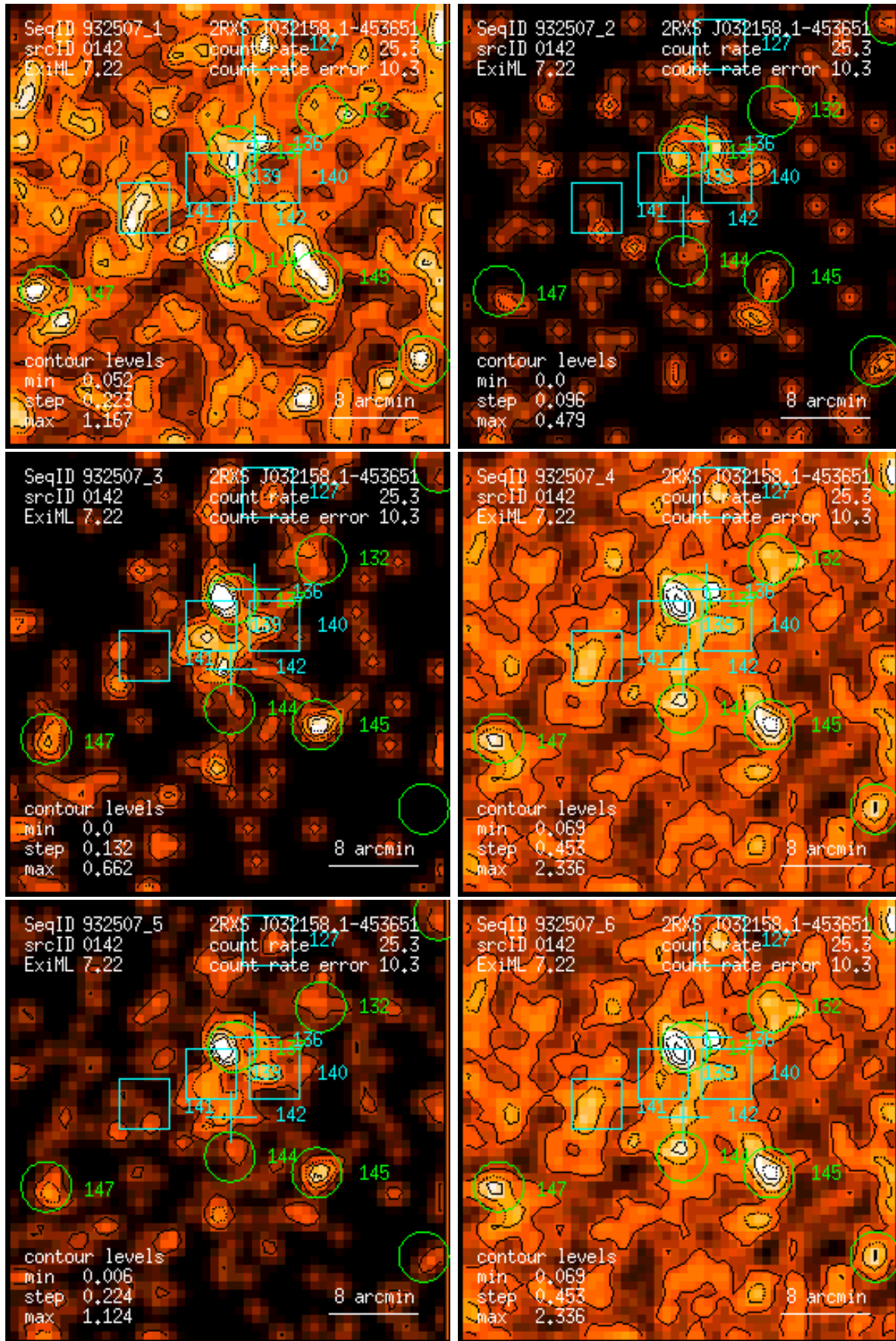
Figure 142: RASS 932507: detection 0142: band rate images, Gaussian filter: (1) PSPC channels 11 – 41, (2) 52 – 90, (3) 91 – 201, (4) 11 – 235, (5) 52 – 201, (6) 11 – 201. Broad band rates in counts/ks. Band rate contour levels in counts/ks/arcmin 2 .
