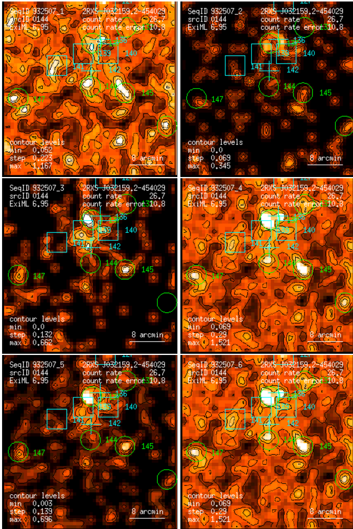
Figure 144: RASS 932507: detection 0144: band rate images, Gaussian filter: (1) PSPC channels 11 – 41, (2) 52 – 90, (3) 91 – 201, (4) 11 – 235, (5) 52 – 201, (6) 11 – 201. Broad band rates in counts/ks. Band rate contour levels in counts/ks/arcmin 2 .
