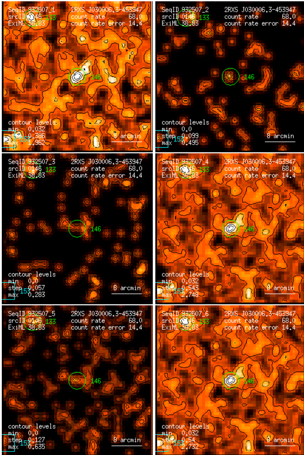
Figure 146: RASS 932507: detection 0146: band rate images, Gaussian filter: (1) PSPC channels 11 – 41, (2) 52 – 90, (3) 91 – 201, (4) 11 – 235, (5) 52 – 201, (6) 11 – 201. Broad band rates in counts/ks. Band rate contour levels in counts/ks/arcmin 2 .
