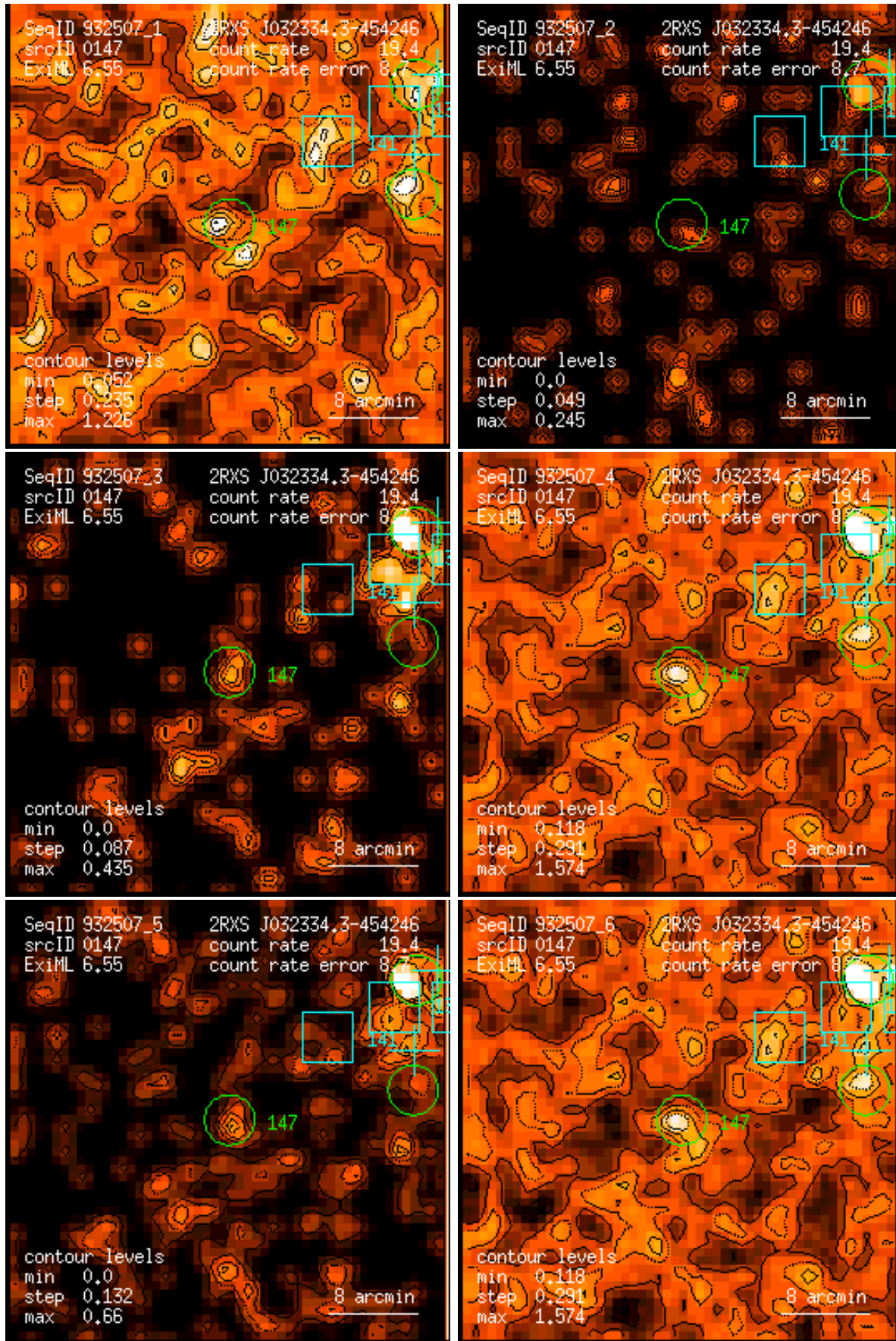
Figure 147: RASS 932507: detection 0147: band rate images, Gaussian filter: (1) PSPC channels 11 – 41, (2) 52 – 90, (3) 91 – 201, (4) 11 – 235, (5) 52 – 201, (6) 11 – 201. Broad band rates in counts/ks. Band rate contour levels in counts/ks/arcmin 2 .
