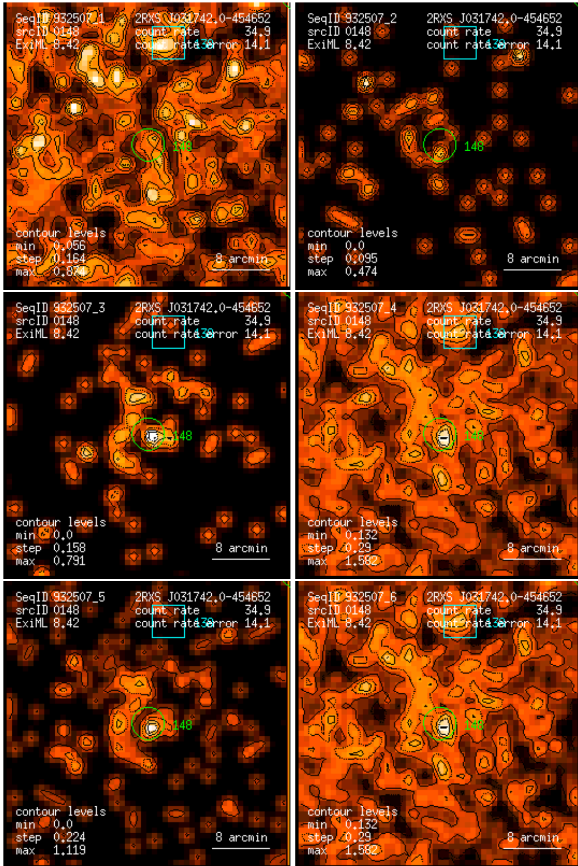
Figure 148: RASS 932507: detection 0148: band rate images, Gaussian filter: (1) PSPC channels 11 – 41, (2) 52 – 90, (3) 91 – 201, (4) 11 – 235, (5) 52 – 201, (6) 11 – 201. Broad band rates in counts/ks. Band rate contour levels in counts/ks/arcmin 2 .
