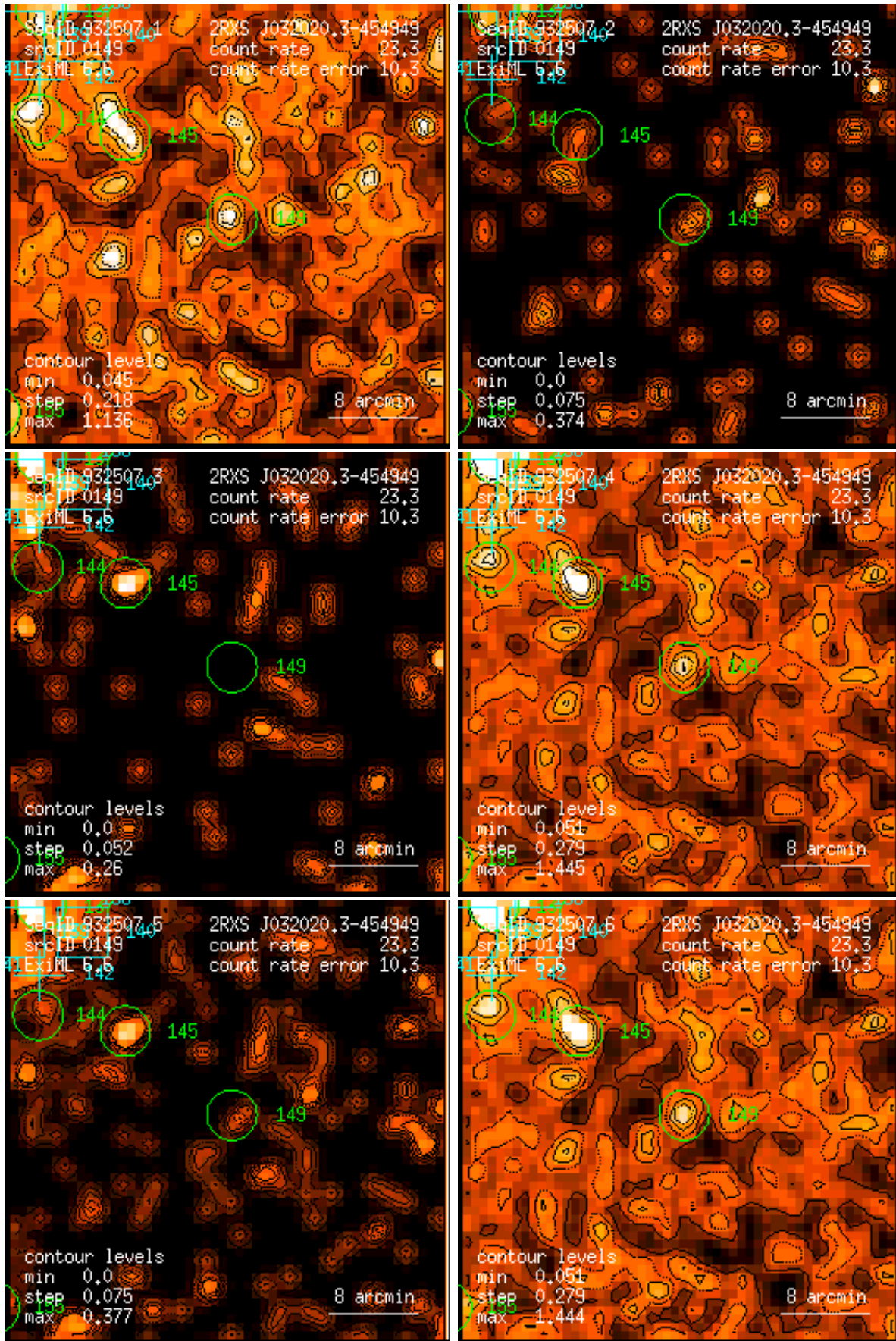
Figure 149: RASS 932507: detection 0149: band rate images, Gaussian filter: (1) PSPC channels 11 – 41, (2) 52 – 90, (3) 91 – 201, (4) 11 – 235, (5) 52 – 201, (6) 11 – 201. Broad band rates in counts/ks. Band rate contour levels in counts/ks/arcmin 2 .
