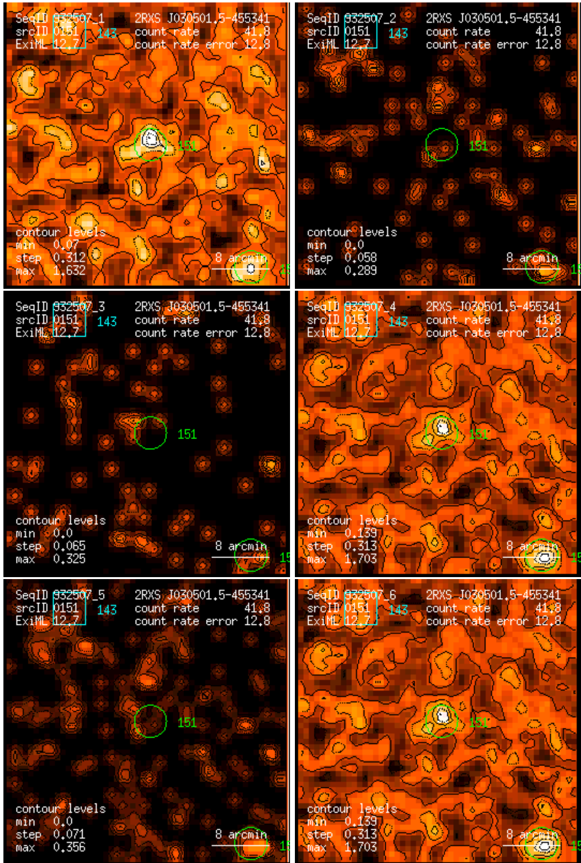
Figure 151: RASS 932507: detection 0151: band rate images, Gaussian filter: (1) PSPC channels 11 – 41, (2) 52 – 90, (3) 91 – 201, (4) 11 – 235, (5) 52 – 201, (6) 11 – 201. Broad band rates in counts/ks. Band rate contour levels in counts/ks/arcmin 2 .
