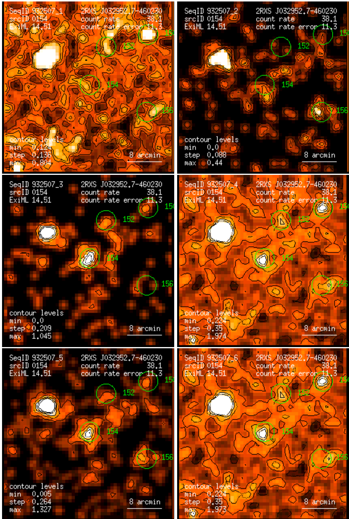
Figure 154: RASS 932507: detection 0154: band rate images, Gaussian filter: (1) PSPC channels 11 – 41, (2) 52 – 90, (3) 91 – 201, (4) 11 – 235, (5) 52 – 201, (6) 11 – 201. Broad band rates in counts/ks. Band rate contour levels in counts/ks/arcmin 2 .
