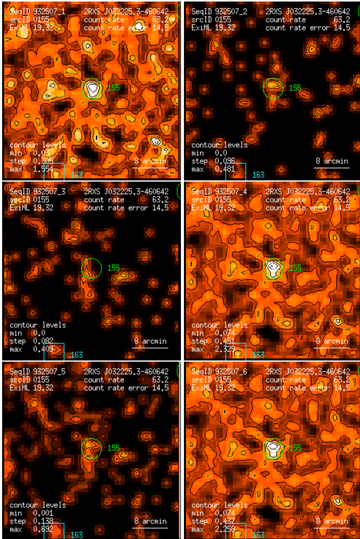
Figure 155: RASS 932507: detection 0155: band rate images, Gaussian filter: (1) PSPC channels 11 – 41, (2) 52 – 90, (3) 91 – 201, (4) 11 – 235, (5) 52 – 201, (6) 11 – 201. Broad band rates in counts/ks. Band rate contour levels in counts/ks/arcmin 2 .
