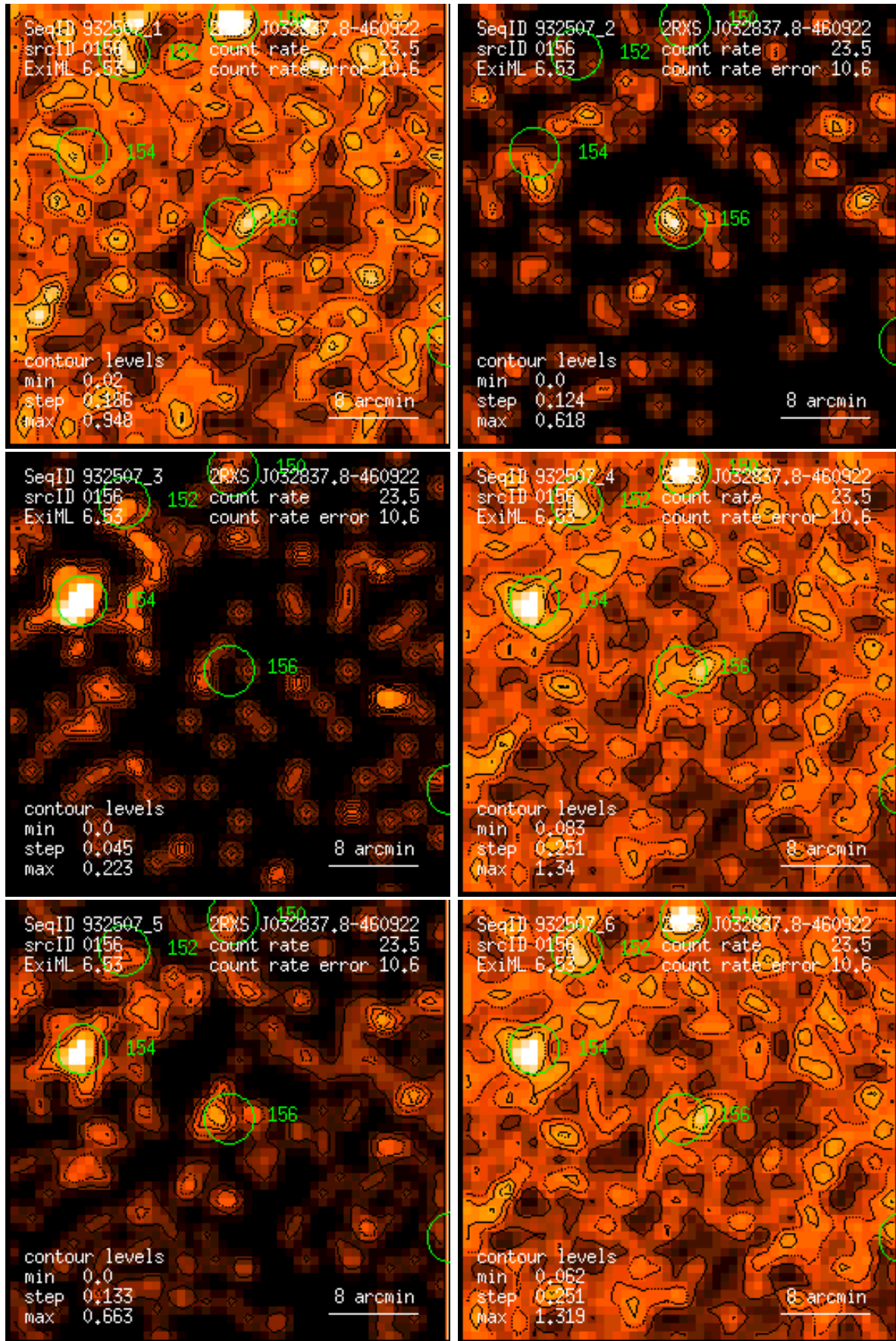
Figure 156: RASS 932507: detection 0156: band rate images, Gaussian filter: (1) PSPC channels 11 – 41, (2) 52 – 90, (3) 91 – 201, (4) 11 – 235, (5) 52 – 201, (6) 11 – 201. Broad band rates in counts/ks. Band rate contour levels in counts/ks/arcmin 2 .
