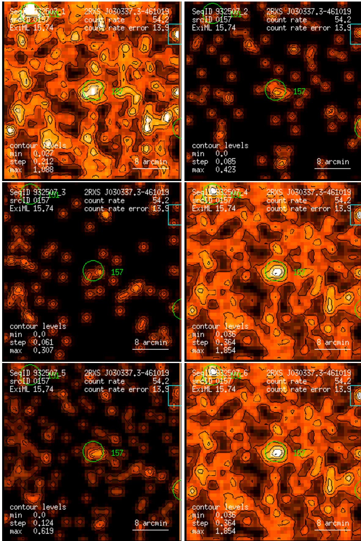
Figure 157: RASS 932507: detection 0157: band rate images, Gaussian filter: (1) PSPC channels 11 – 41, (2) 52 – 90, (3) 91 – 201, (4) 11 – 235, (5) 52 – 201, (6) 11 – 201. Broad band rates in counts/ks. Band rate contour levels in counts/ks/arcmin 2 .
