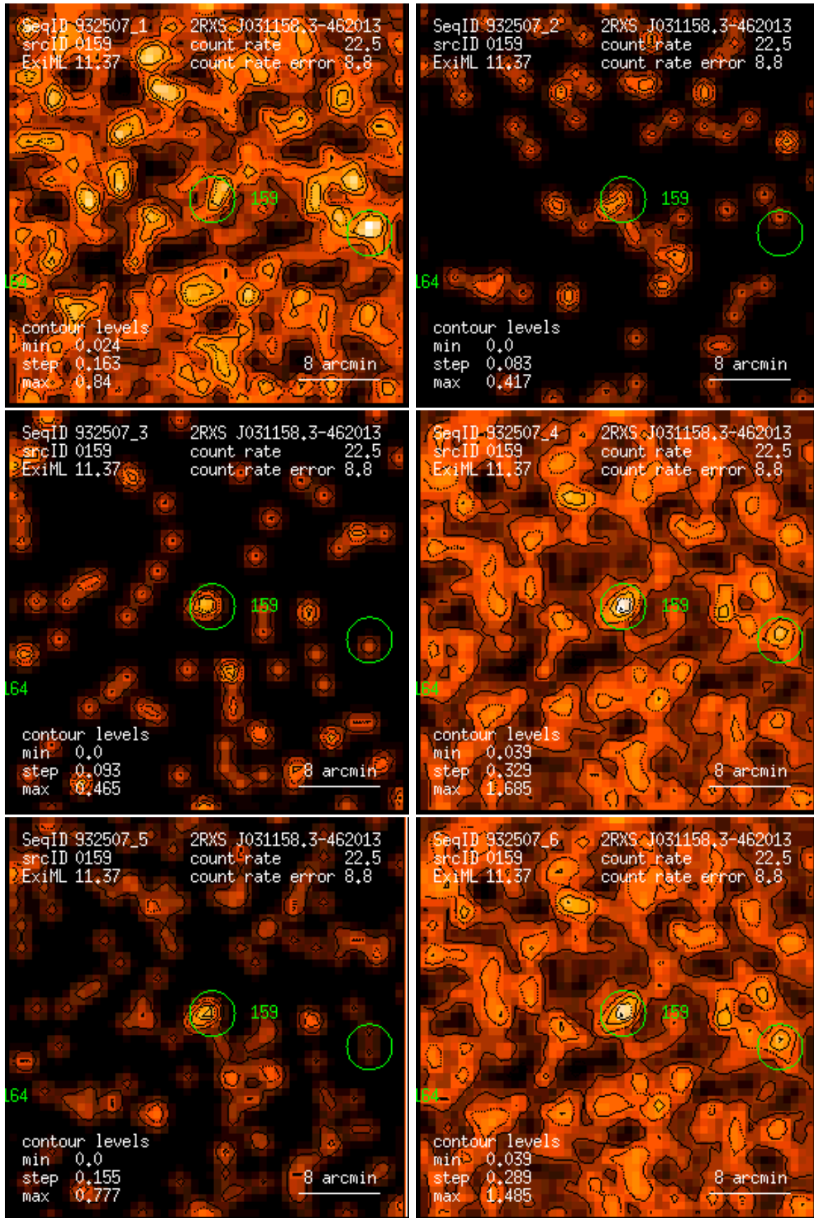
Figure 159: RASS 932507: detection 0159: band rate images, Gaussian filter: (1) PSPC channels 11 – 41, (2) 52 – 90, (3) 91 – 201, (4) 11 – 235, (5) 52 – 201, (6) 11 – 201. Broad band rates in counts/ks. Band rate contour levels in counts/ks/arcmin 2 .
