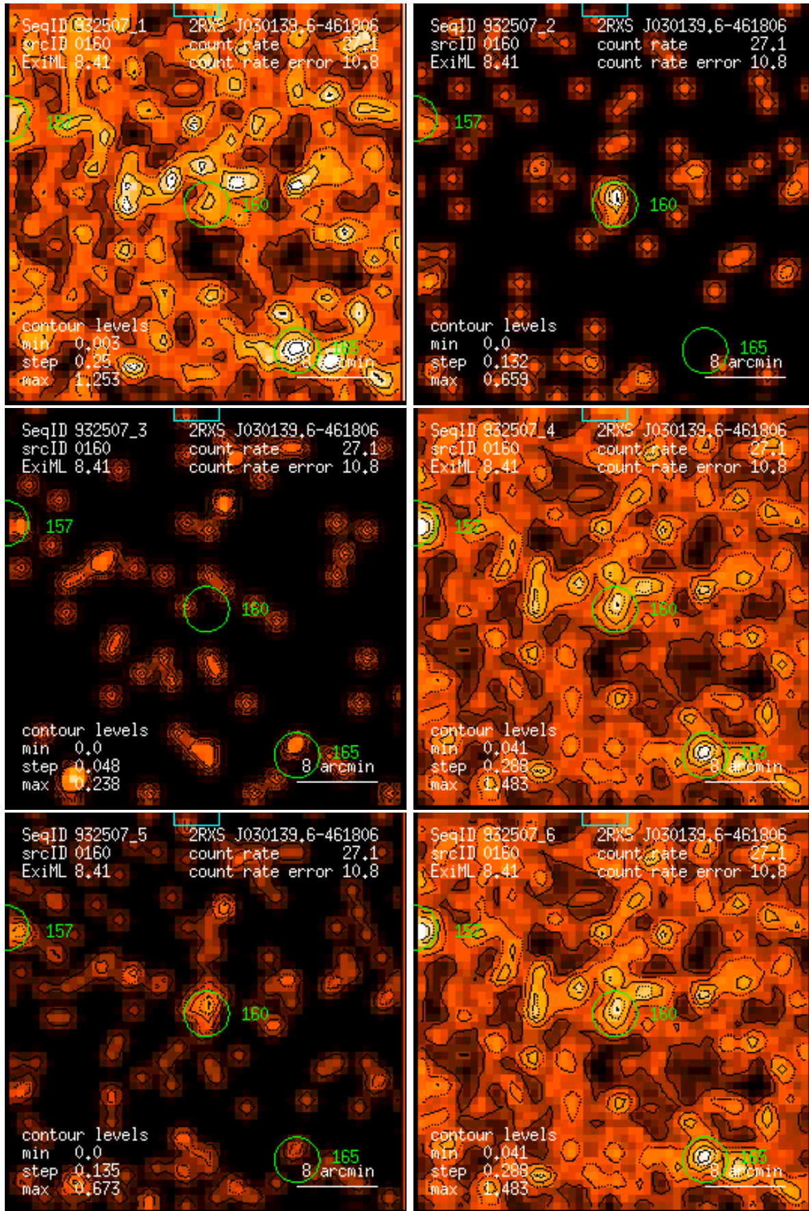
Figure 160: RASS 932507: detection 0160: band rate images, Gaussian filter: (1) PSPC channels 11 – 41, (2) 52 – 90, (3) 91 – 201, (4) 11 – 235, (5) 52 – 201, (6) 11 – 201. Broad band rates in counts/ks. Band rate contour levels in counts/ks/arcmin 2 .
