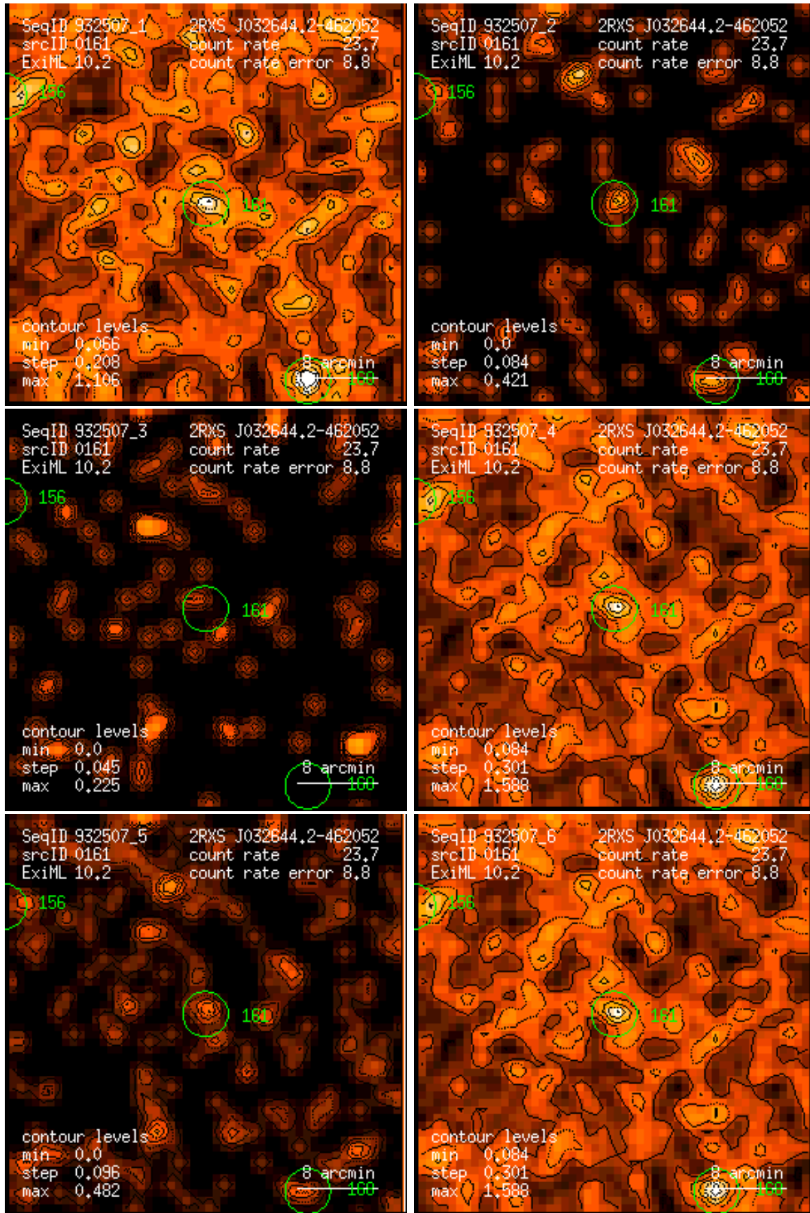
Figure 161: RASS 932507: detection 0161: band rate images, Gaussian filter: (1) PSPC channels 11 – 41, (2) 52 – 90, (3) 91 – 201, (4) 11 – 235, (5) 52 – 201, (6) 11 – 201. Broad band rates in counts/ks. Band rate contour levels in counts/ks/arcmin 2 .
