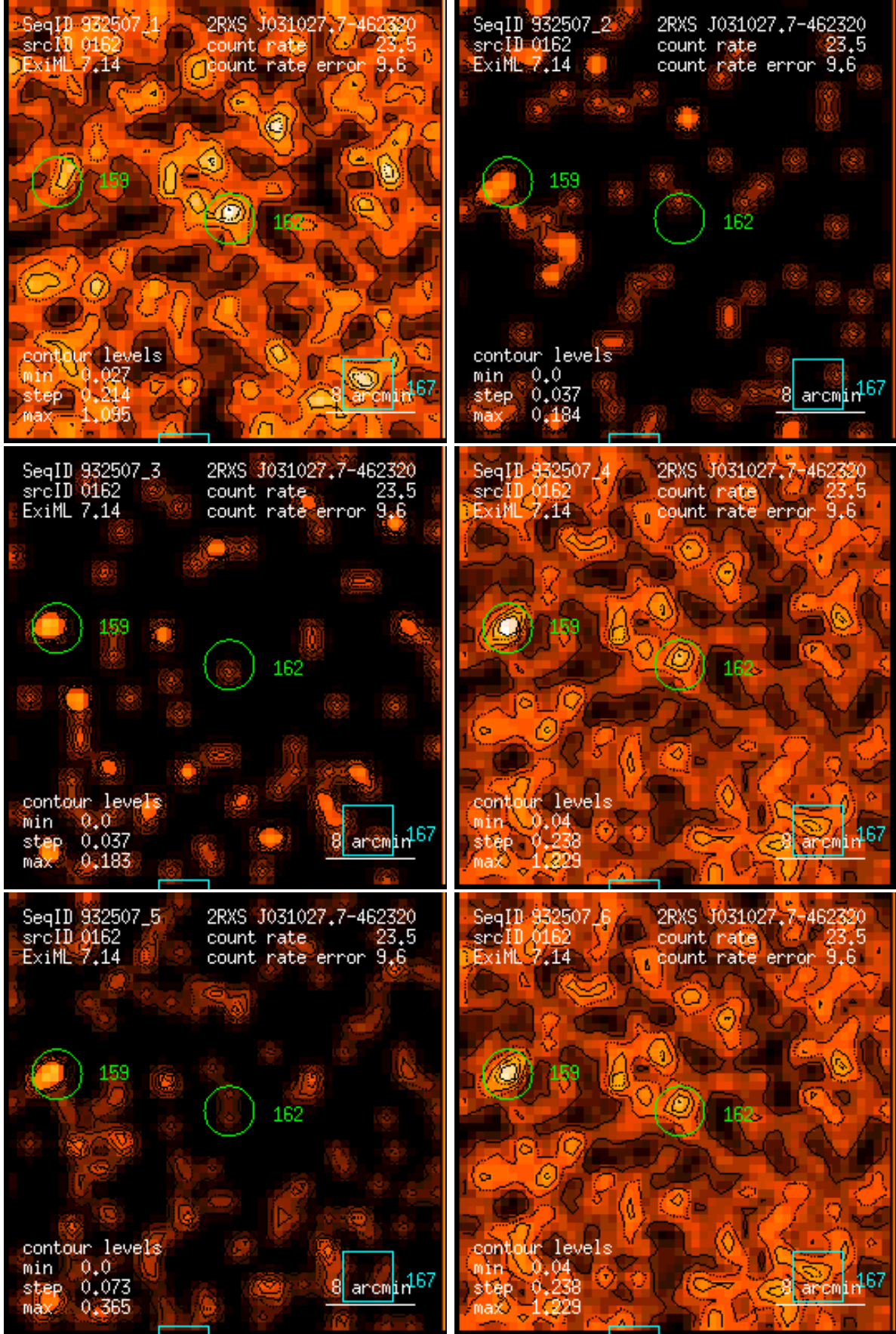
Figure 162: RASS 932507: detection 0162: band rate images, Gaussian filter: (1) PSPC channels 11 – 41, (2) 52 – 90, (3) 91 – 201, (4) 11 – 235, (5) 52 – 201, (6) 11 – 201. Broad band rates in counts/ks. Band rate contour levels in counts/ks/arcmin 2 .
