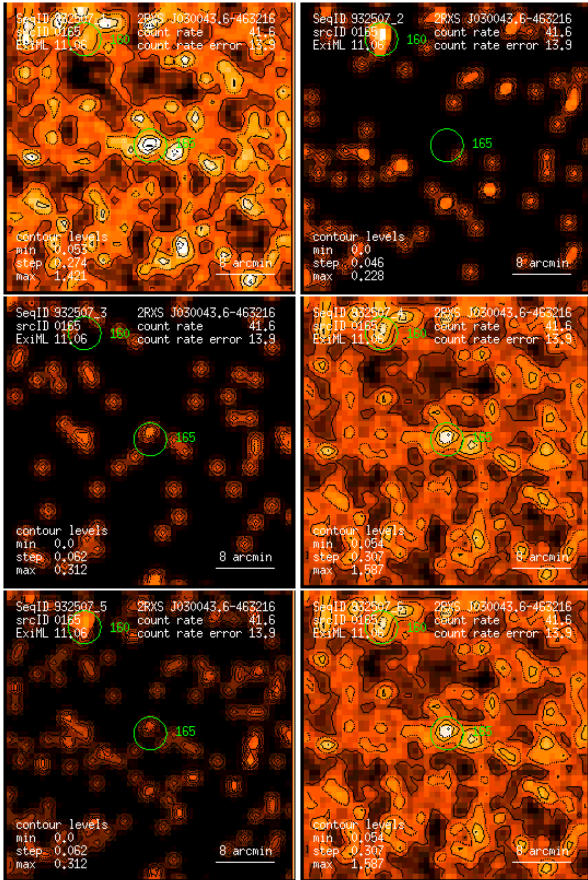
Figure 165: RASS 932507: detection 0165: band rate images, Gaussian filter: (1) PSPC channels 11 – 41, (2) 52 – 90, (3) 91 – 201, (4) 11 – 235, (5) 52 – 201, (6) 11 – 201. Broad band rates in counts/ks. Band rate contour levels in counts/ks/arcmin 2 .
