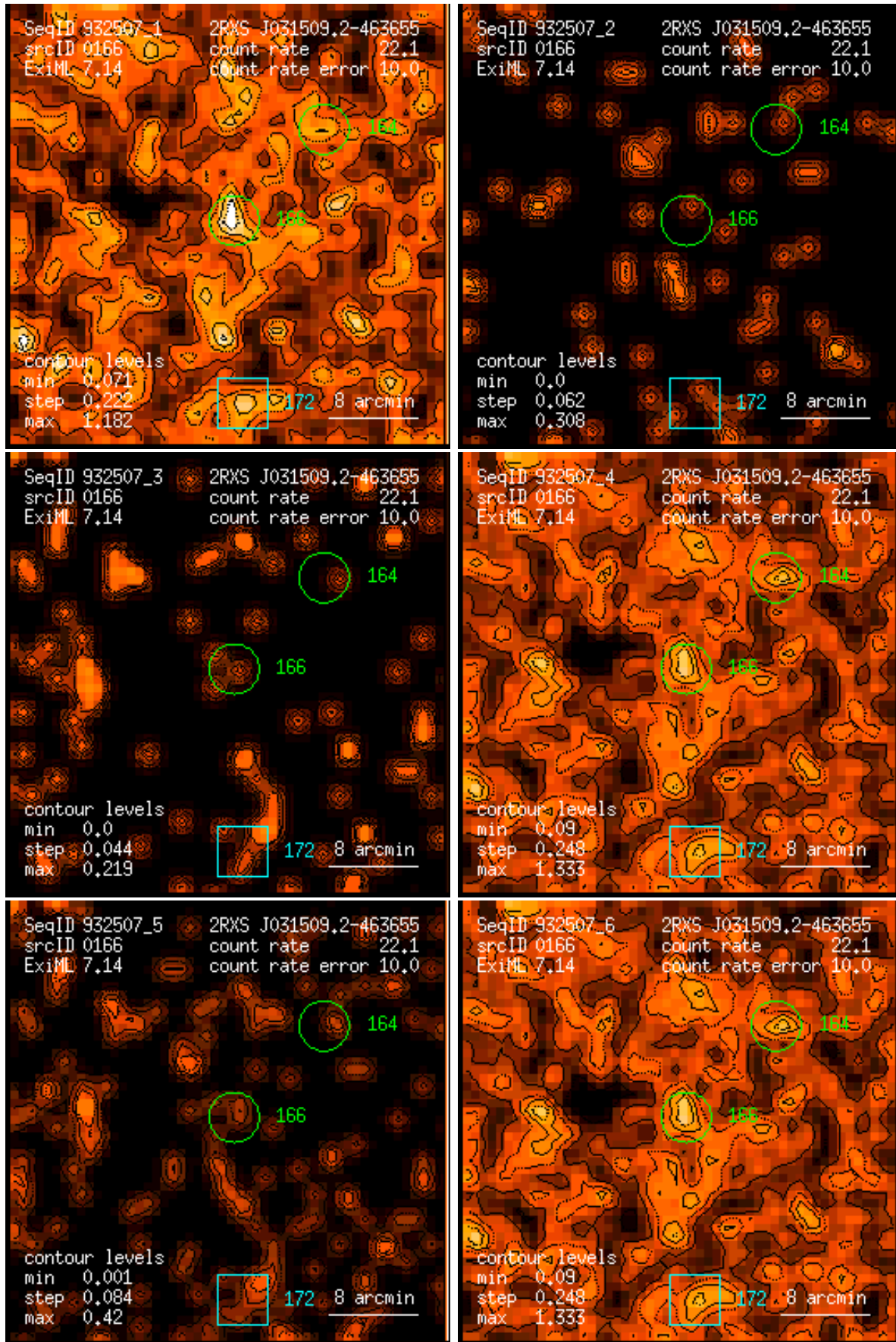
Figure 166: RASS 932507: detection 0166: band rate images, Gaussian filter: (1) PSPC channels 11 – 41, (2) 52 – 90, (3) 91 – 201, (4) 11 – 235, (5) 52 – 201, (6) 11 – 201. Broad band rates in counts/ks. Band rate contour levels in counts/ks/arcmin 2 .
