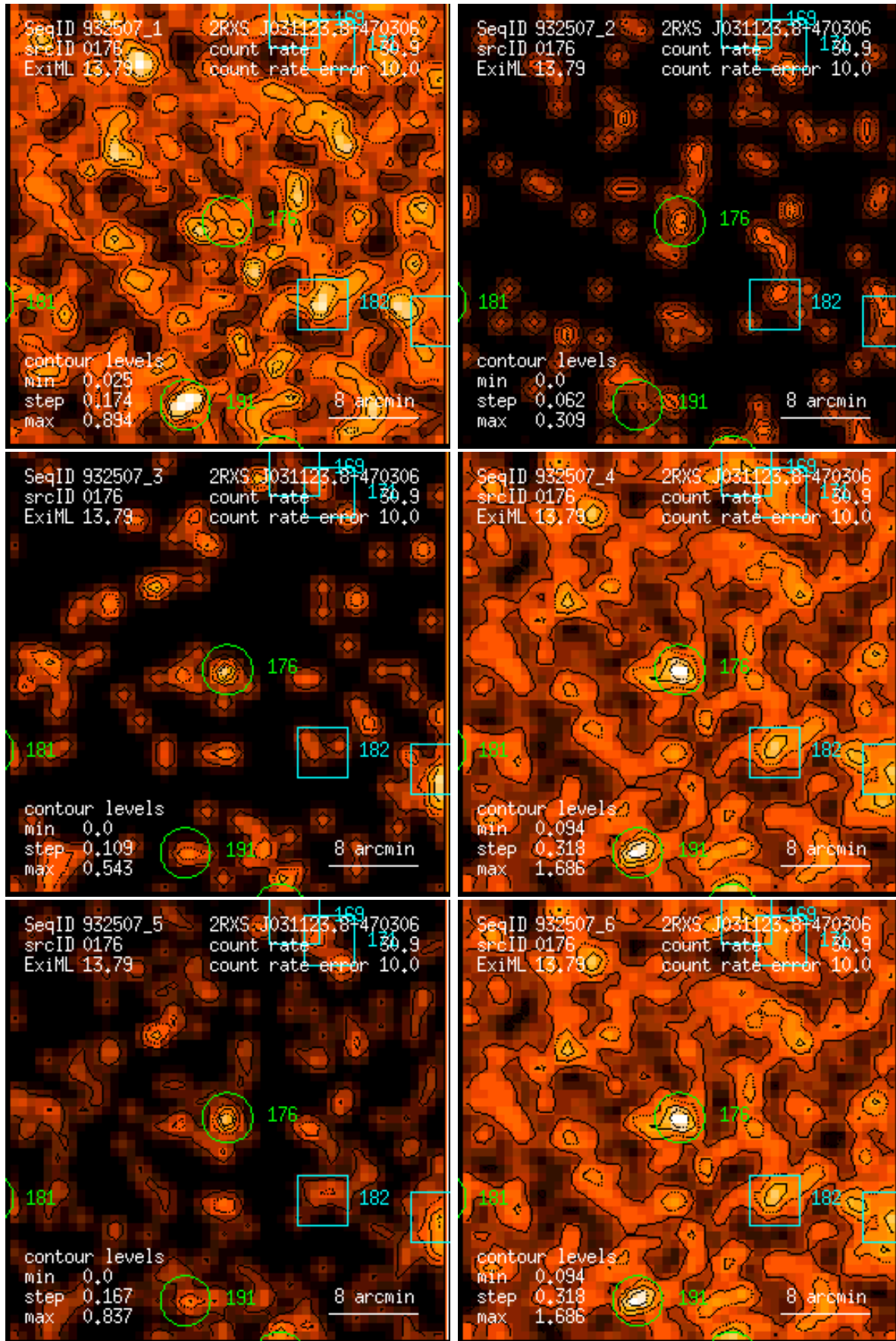
Figure 176: RASS 932507: detection 0176: band rate images, Gaussian filter: (1) PSPC channels 11 – 41, (2) 52 – 90, (3) 91 – 201, (4) 11 – 235, (5) 52 – 201, (6) 11 – 201. Broad band rates in counts/ks. Band rate contour levels in counts/ks/arcmin 2 .
