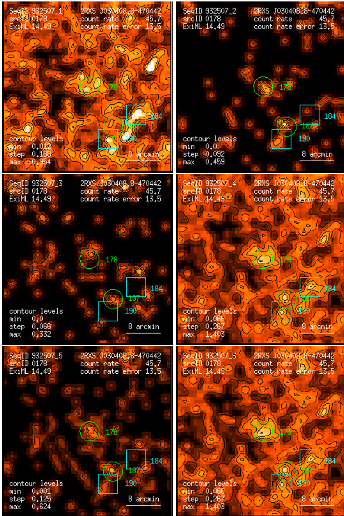
Figure 178: RASS 932507: detection 0178: band rate images, Gaussian filter: (1) PSPC channels 11 – 41, (2) 52 – 90, (3) 91 – 201, (4) 11 – 235, (5) 52 – 201, (6) 11 – 201. Broad band rates in counts/ks. Band rate contour levels in counts/ks/arcmin 2 .
