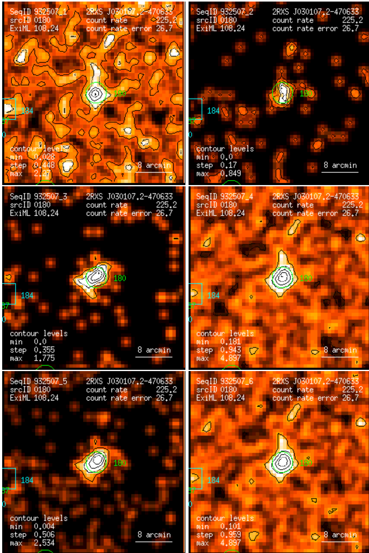
Figure 180: RASS 932507: detection 0180: band rate images, Gaussian filter: (1) PSPC channels 11 – 41, (2) 52 – 90, (3) 91 – 201, (4) 11 – 235, (5) 52 – 201, (6) 11 – 201. Broad band rates in counts/ks. Band rate contour levels in counts/ks/arcmin 2 .
