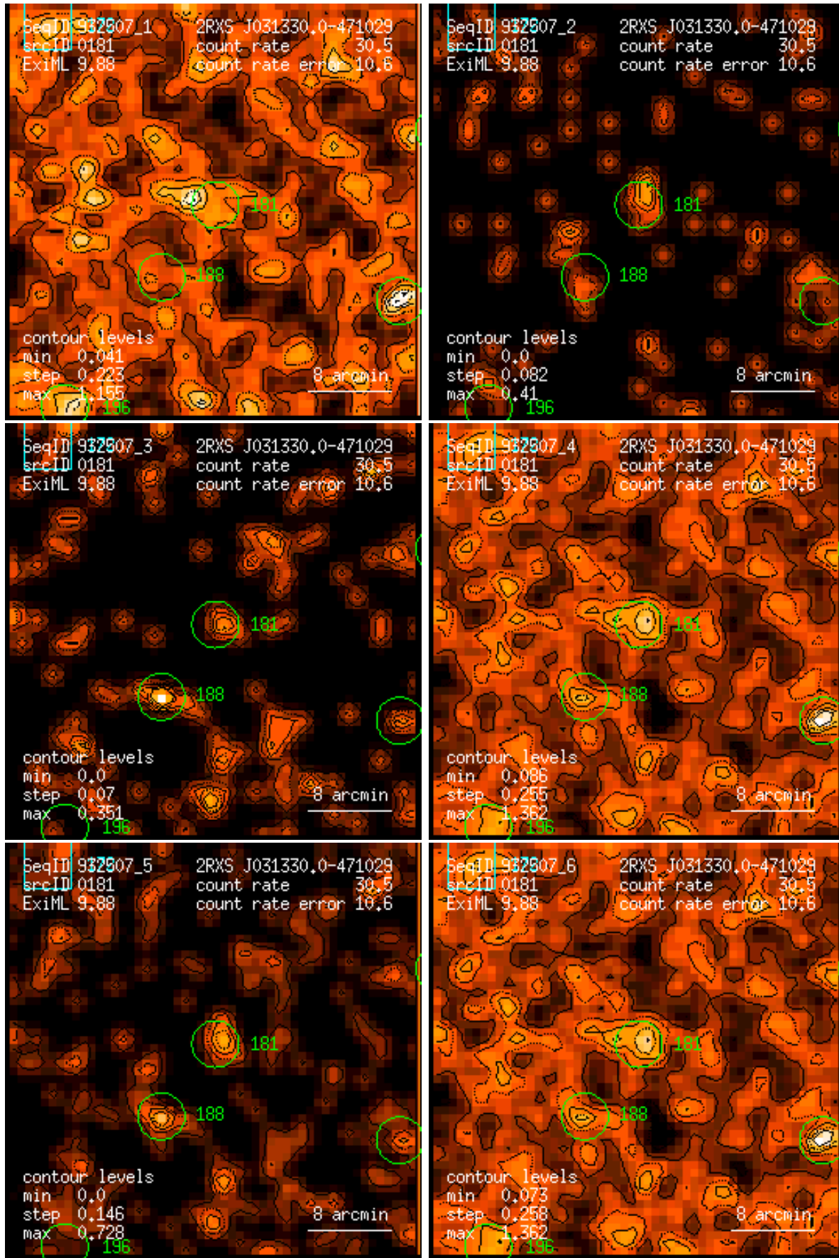
Figure 181: RASS 932507: detection 0181: band rate images, Gaussian filter: (1) PSPC channels 11 – 41, (2) 52 – 90, (3) 91 – 201, (4) 11 – 235, (5) 52 – 201, (6) 11 – 201. Broad band rates in counts/ks. Band rate contour levels in counts/ks/arcmin 2 .
