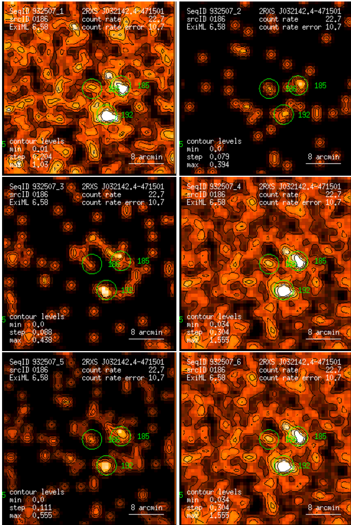
Figure 186: RASS 932507: detection 0186: band rate images, Gaussian filter: (1) PSPC channels 11 – 41, (2) 52 – 90, (3) 91 – 201, (4) 11 – 235, (5) 52 – 201, (6) 11 – 201. Broad band rates in counts/ks. Band rate contour levels in counts/ks/arcmin 2 .
