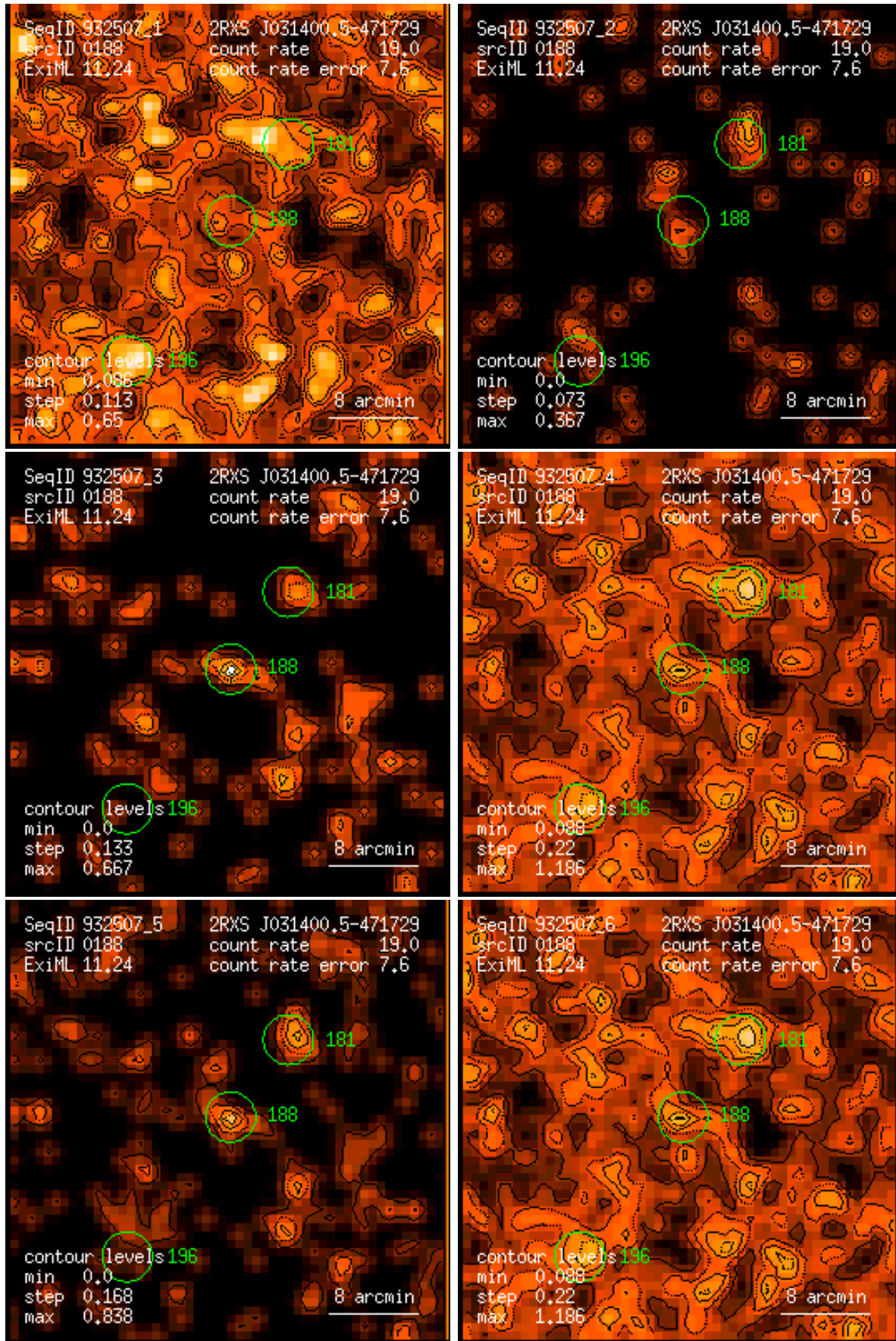
Figure 188: RASS 932507: detection 0188: band rate images, Gaussian filter: (1) PSPC channels 11 – 41, (2) 52 – 90, (3) 91 – 201, (4) 11 – 235, (5) 52 – 201, (6) 11 – 201. Broad band rates in counts/ks. Band rate contour levels in counts/ks/arcmin 2 .
