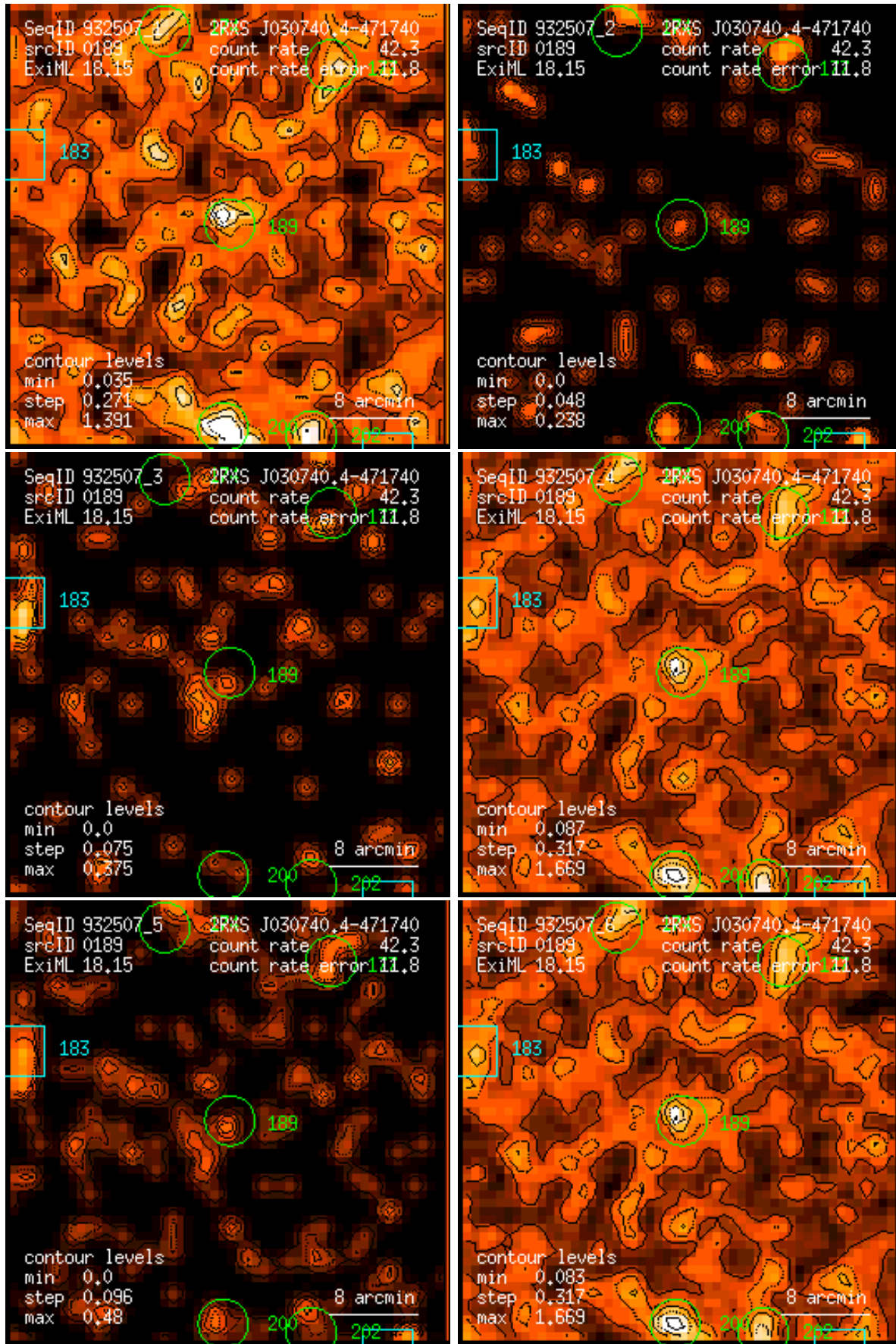
Figure 189: RASS 932507: detection 0189: band rate images, Gaussian filter: (1) PSPC channels 11 – 41, (2) 52 – 90, (3) 91 – 201, (4) 11 – 235, (5) 52 – 201, (6) 11 – 201. Broad band rates in counts/ks. Band rate contour levels in counts/ks/arcmin 2 .
