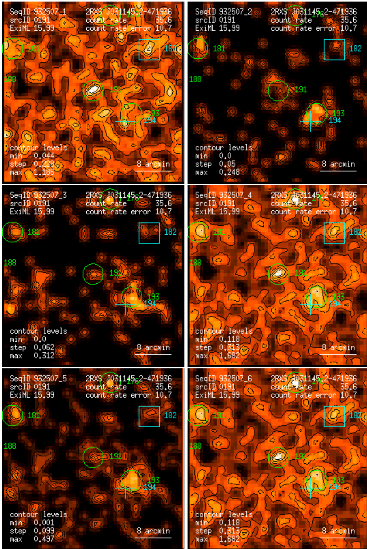
Figure 191: RASS 932507: detection 0191: band rate images, Gaussian filter: (1) PSPC channels 11 – 41, (2) 52 – 90, (3) 91 – 201, (4) 11 – 235, (5) 52 – 201, (6) 11 – 201. Broad band rates in counts/ks. Band rate contour levels in counts/ks/arcmin 2 .
