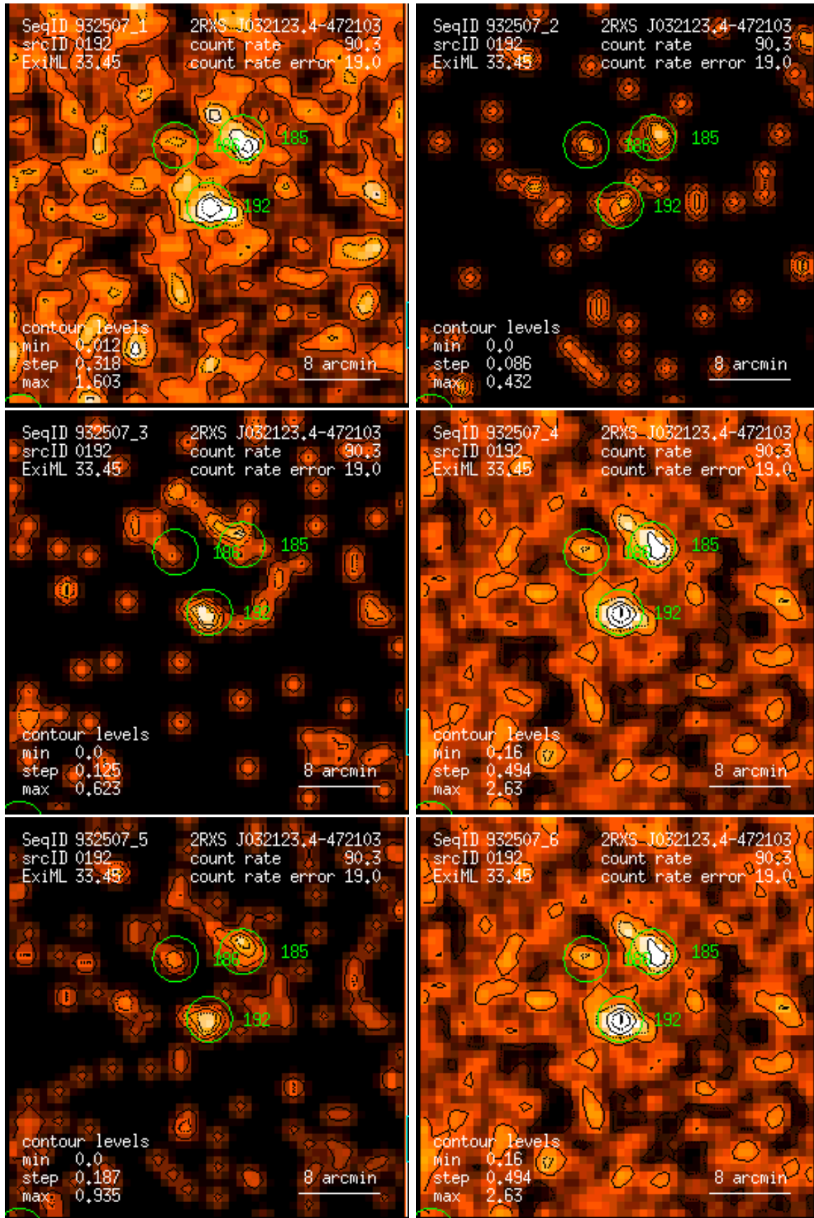
Figure 192: RASS 932507: detection 0192: band rate images, Gaussian filter: (1) PSPC channels 11 – 41, (2) 52 – 90, (3) 91 – 201, (4) 11 – 235, (5) 52 – 201, (6) 11 – 201. Broad band rates in counts/ks. Band rate contour levels in counts/ks/arcmin 2 .
