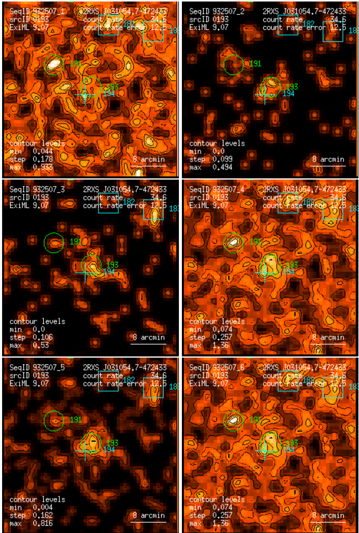
Figure 193: RASS 932507: detection 0193: band rate images, Gaussian filter: (1) PSPC channels 11 – 41, (2) 52 – 90, (3) 91 – 201, (4) 11 – 235, (5) 52 – 201, (6) 11 – 201. Broad band rates in counts/ks. Band rate contour levels in counts/ks/arcmin 2 .
