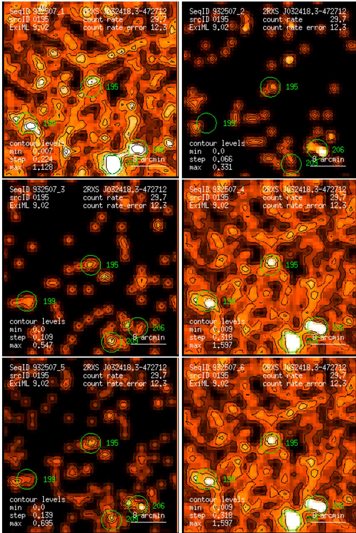
Figure 195: RASS 932507: detection 0195: band rate images, Gaussian filter: (1) PSPC channels 11 – 41, (2) 52 – 90, (3) 91 – 201, (4) 11 – 235, (5) 52 – 201, (6) 11 – 201. Broad band rates in counts/ks. Band rate contour levels in counts/ks/arcmin 2 .
