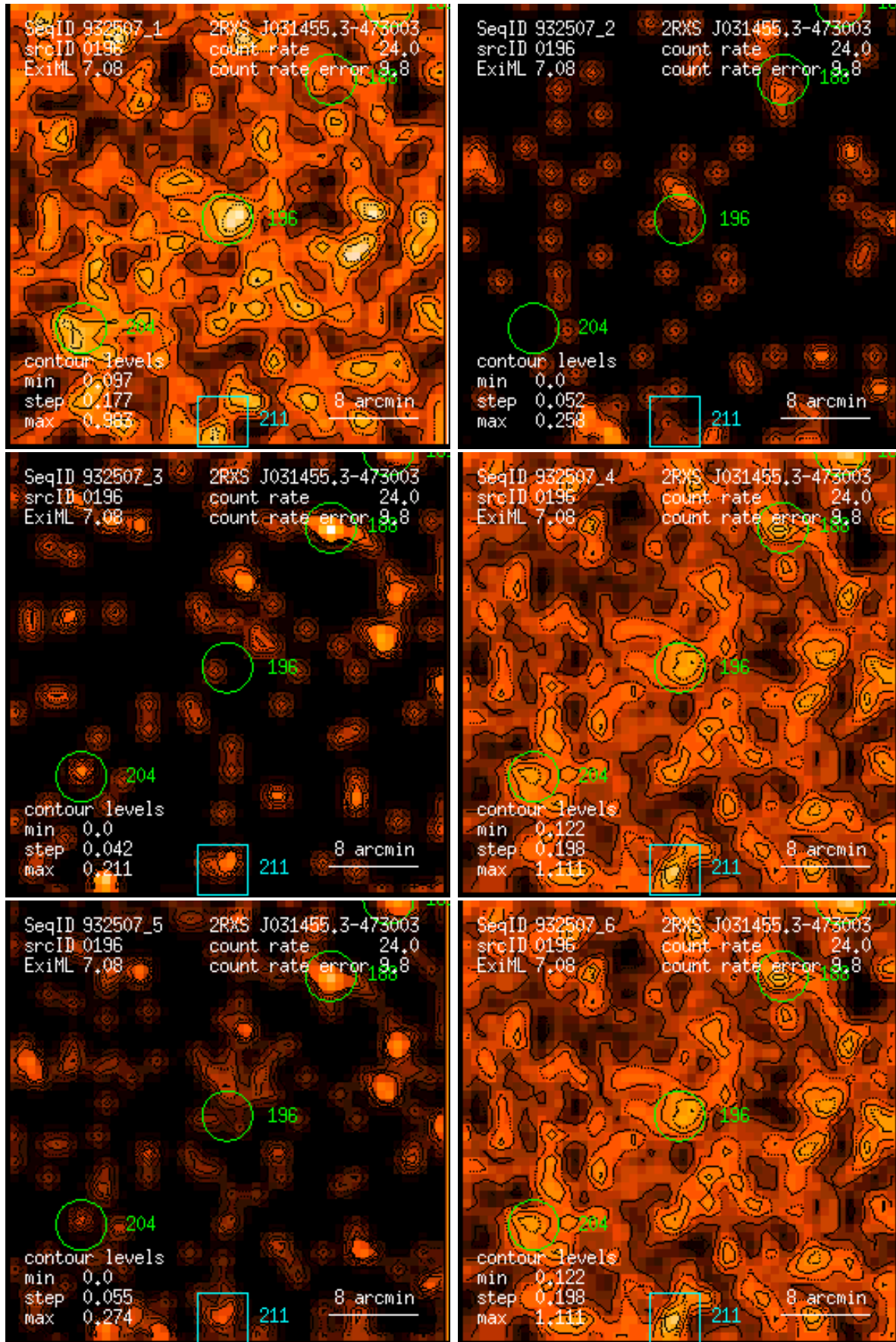
Figure 196: RASS 932507: detection 0196: band rate images, Gaussian filter: (1) PSPC channels 11 – 41, (2) 52 – 90, (3) 91 – 201, (4) 11 – 235, (5) 52 – 201, (6) 11 – 201. Broad band rates in counts/ks. Band rate contour levels in counts/ks/arcmin 2 .
