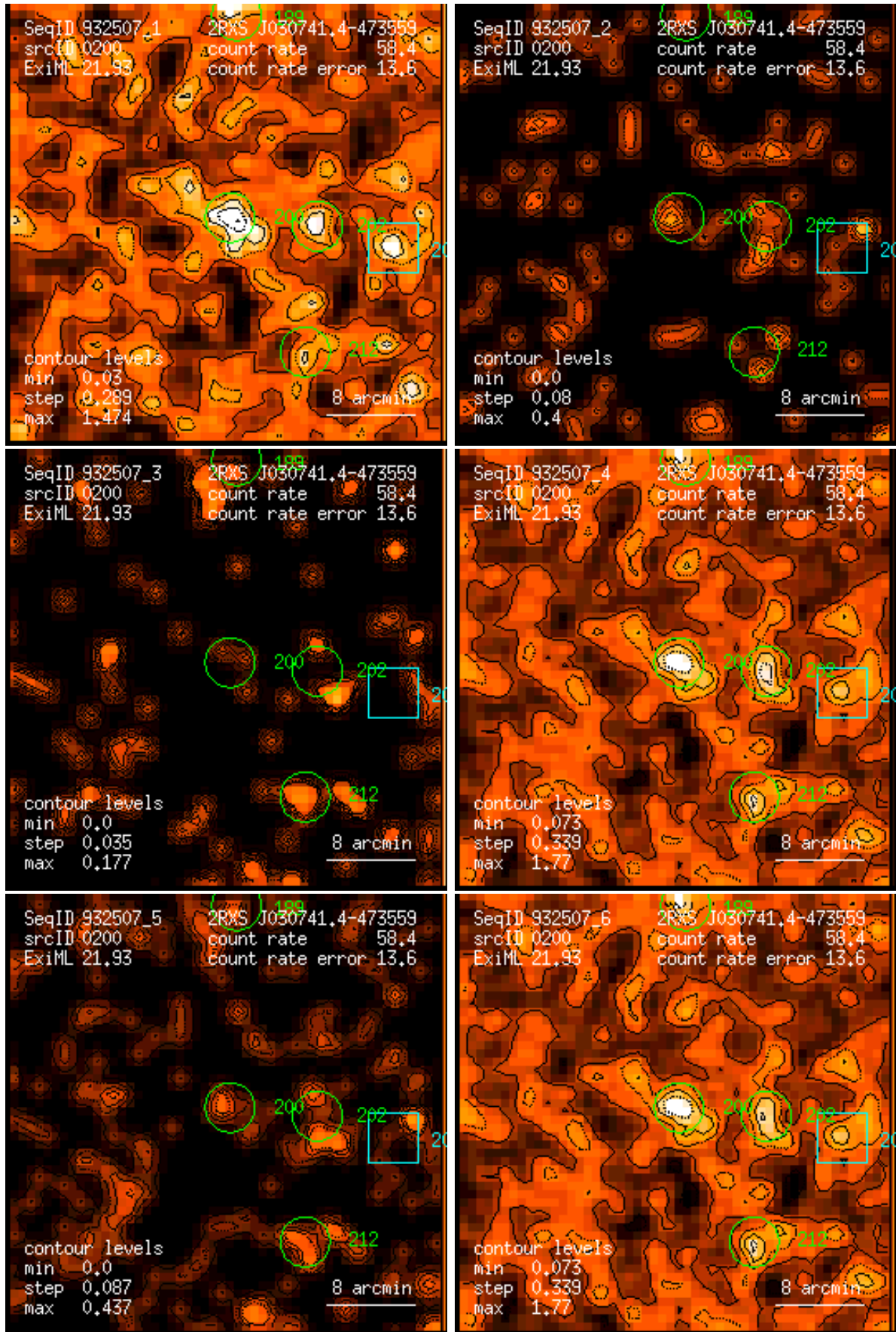
Figure 200: RASS 932507: detection 0200: band rate images, Gaussian filter: (1) PSPC channels 11 – 41, (2) 52 – 90, (3) 91 – 201, (4) 11 – 235, (5) 52 – 201, (6) 11 – 201. Broad band rates in counts/ks. Band rate contour levels in counts/ks/arcmin 2 .
