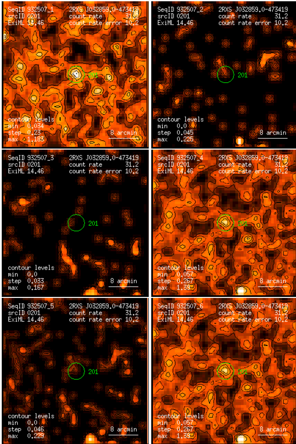
Figure 201: RASS 932507: detection 0201: band rate images, Gaussian filter: (1) PSPC channels 11 – 41, (2) 52 – 90, (3) 91 – 201, (4) 11 – 235, (5) 52 – 201, (6) 11 – 201. Broad band rates in counts/ks. Band rate contour levels in counts/ks/arcmin 2 .
