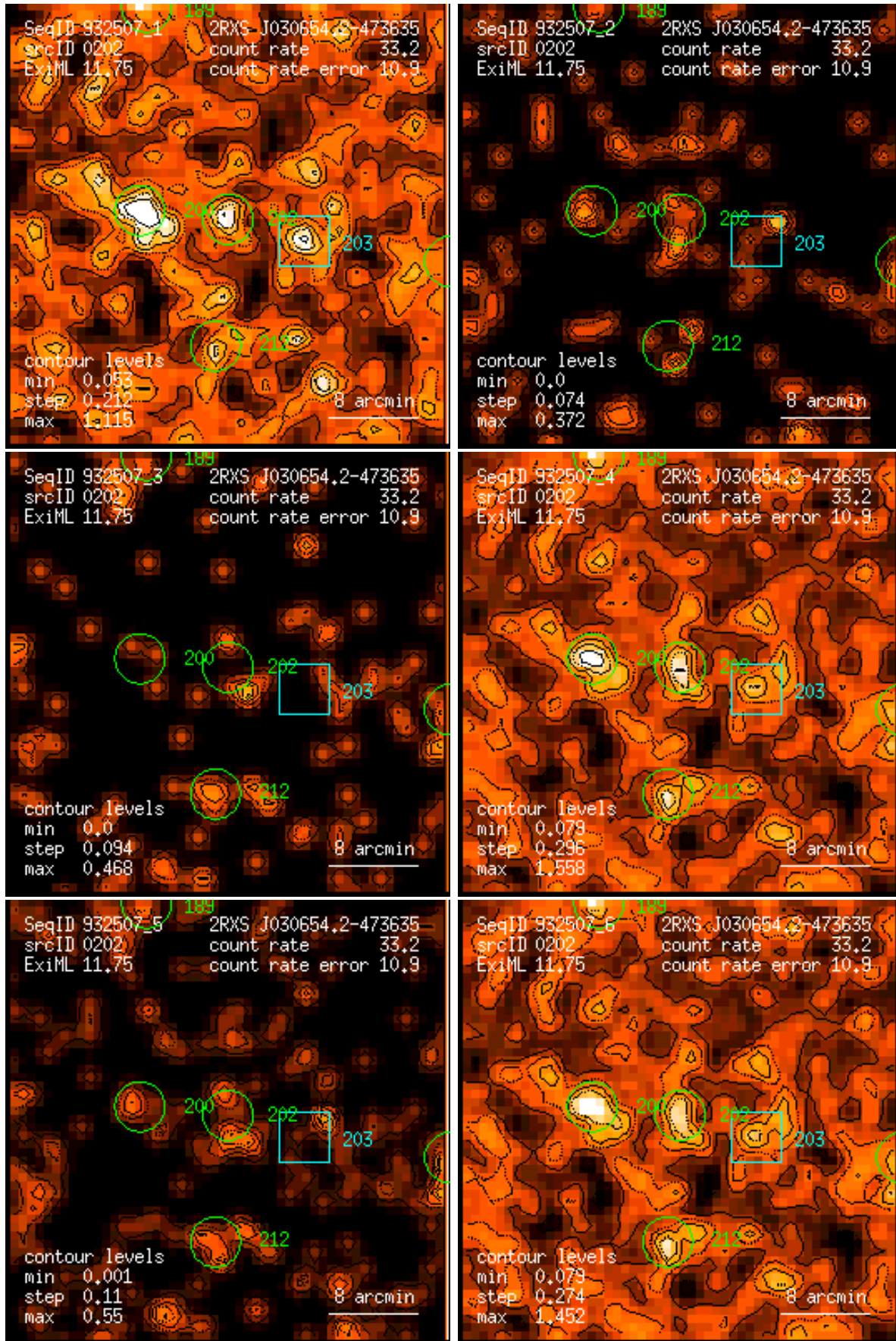
Figure 202: RASS 932507: detection 0202: band rate images, Gaussian filter: (1) PSPC channels 11 – 41, (2) 52 – 90, (3) 91 – 201, (4) 11 – 235, (5) 52 – 201, (6) 11 – 201. Broad band rates in counts/ks. Band rate contour levels in counts/ks/arcmin 2 .
