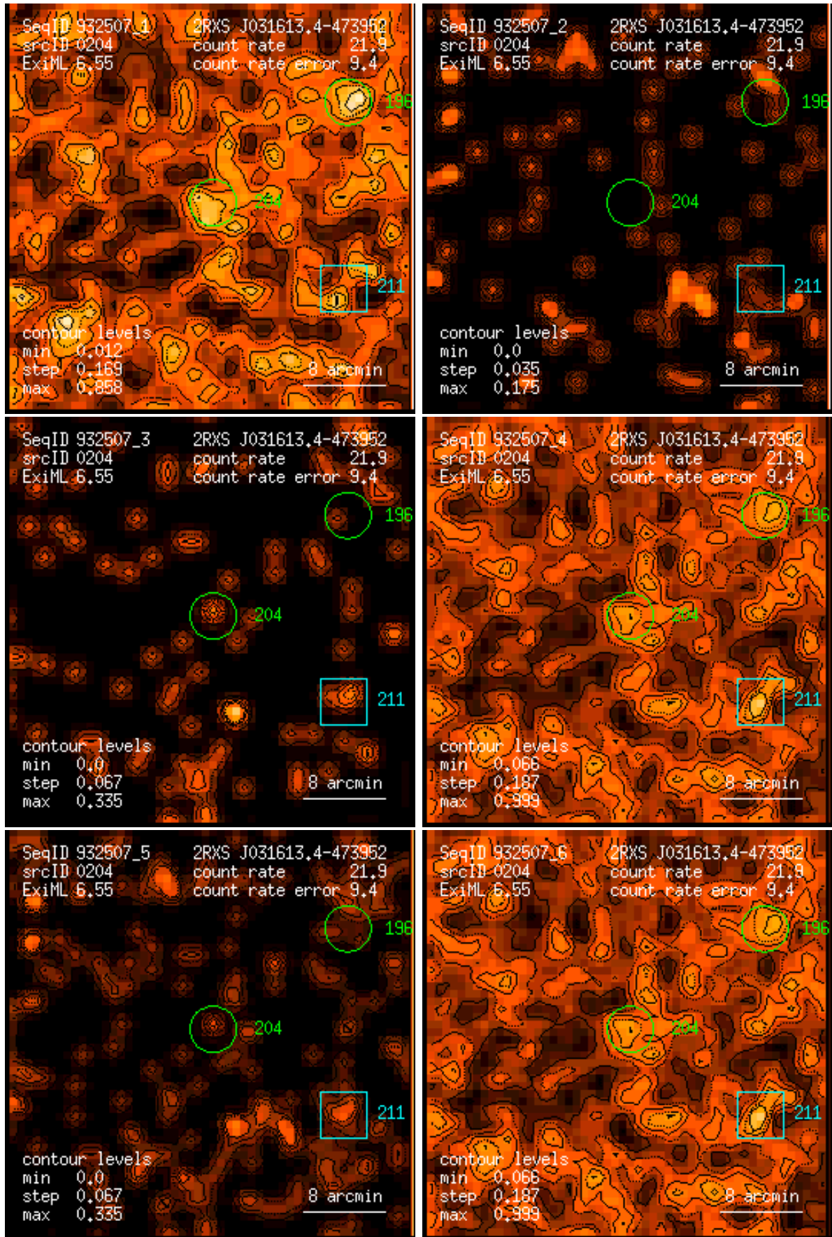
Figure 204: RASS 932507: detection 0204: band rate images, Gaussian filter: (1) PSPC channels 11 – 41, (2) 52 – 90, (3) 91 – 201, (4) 11 – 235, (5) 52 – 201, (6) 11 – 201. Broad band rates in counts/ks. Band rate contour levels in counts/ks/arcmin 2 .
