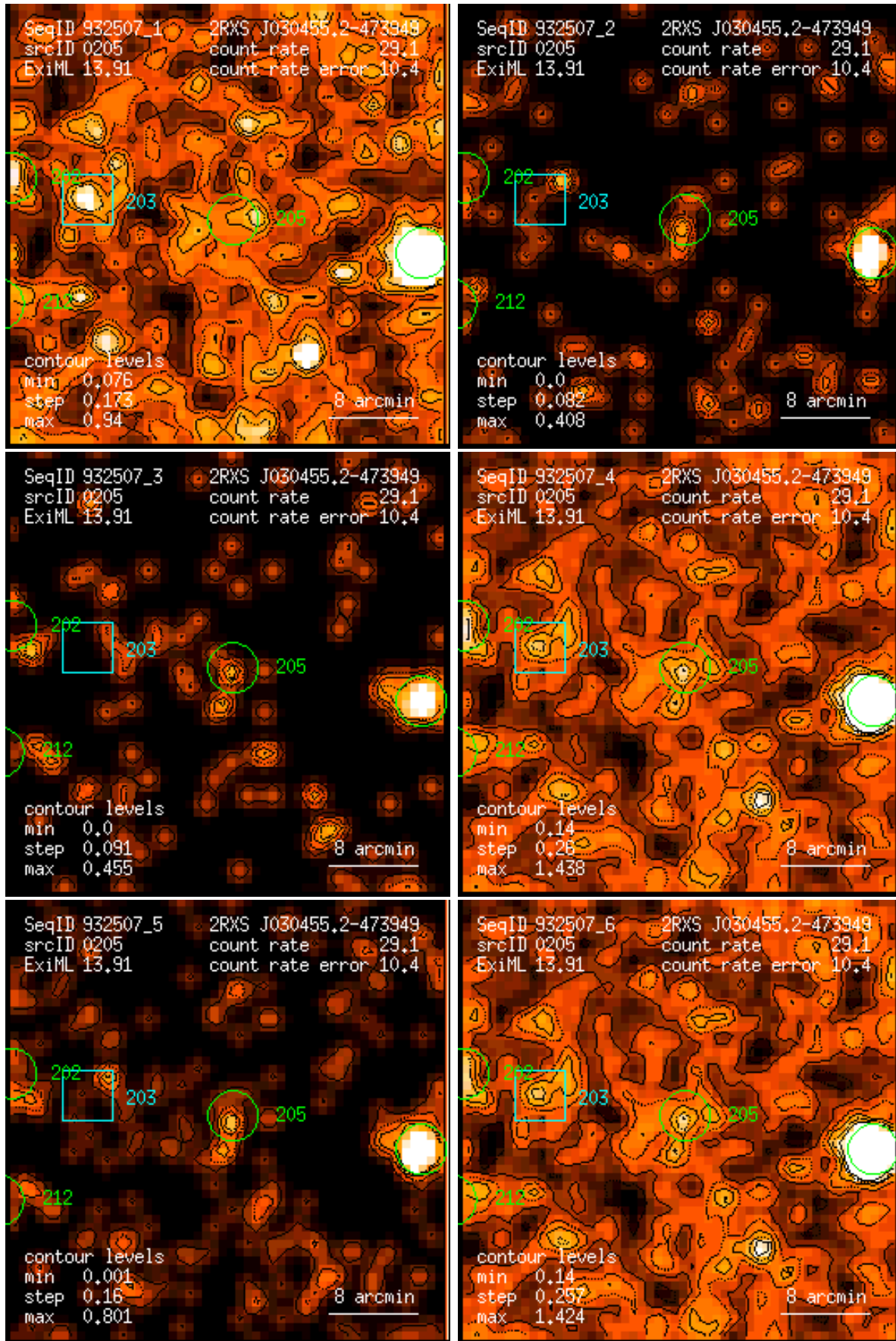
Figure 205: RASS 932507: detection 0205: band rate images, Gaussian filter: (1) PSPC channels 11 – 41, (2) 52 – 90, (3) 91 – 201, (4) 11 – 235, (5) 52 – 201, (6) 11 – 201. Broad band rates in counts/ks. Band rate contour levels in counts/ks/arcmin 2 .
