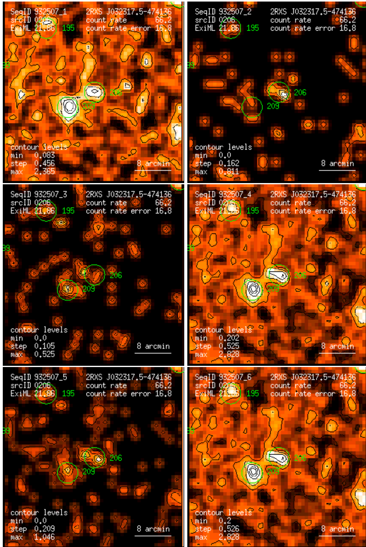
Figure 206: RASS 932507: detection 0206: band rate images, Gaussian filter: (1) PSPC channels 11 – 41, (2) 52 – 90, (3) 91 – 201, (4) 11 – 235, (5) 52 – 201, (6) 11 – 201. Broad band rates in counts/ks. Band rate contour levels in counts/ks/arcmin 2 .
