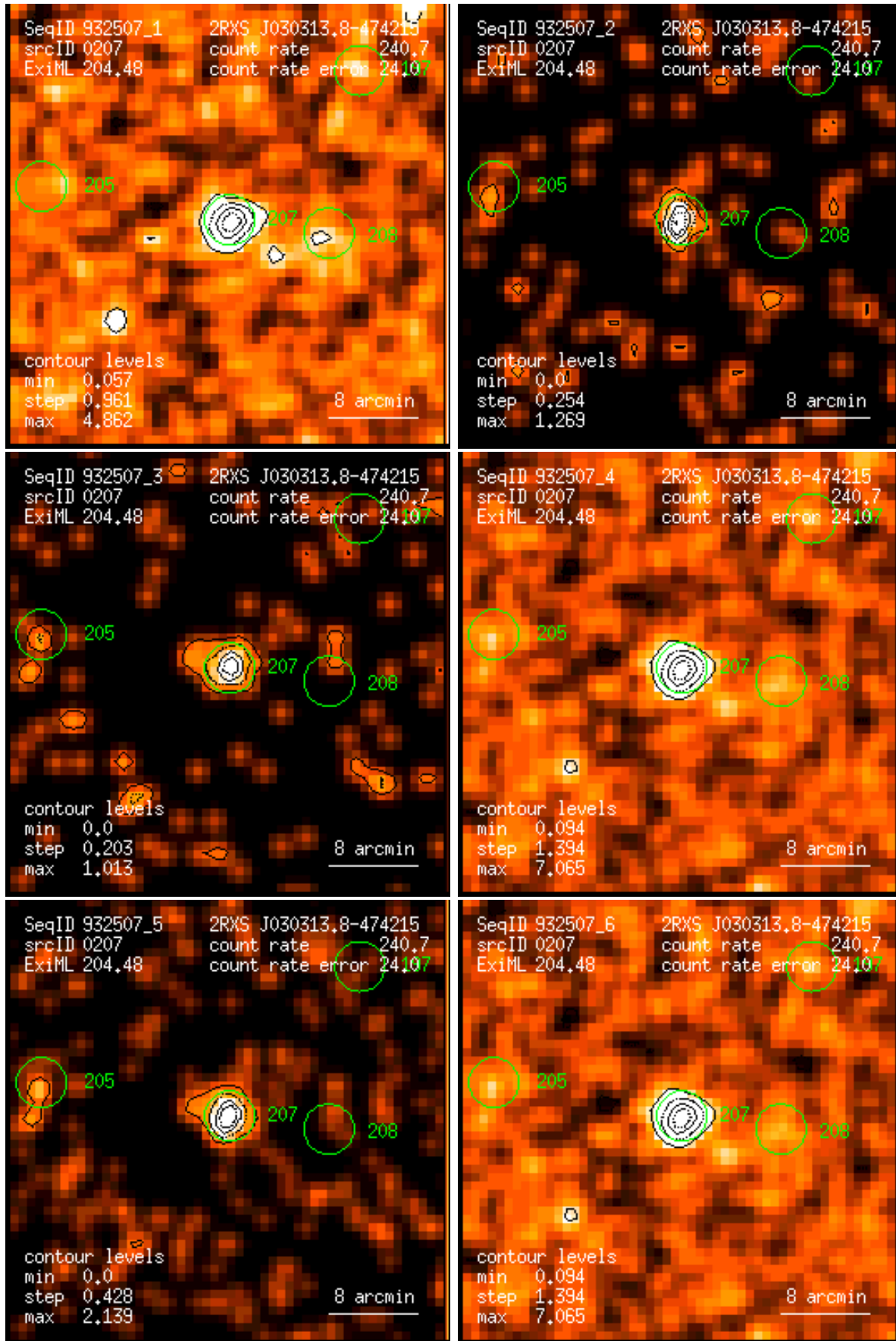
Figure 207: RASS 932507: detection 0207: band rate images, Gaussian filter: (1) PSPC channels 11 – 41, (2) 52 – 90, (3) 91 – 201, (4) 11 – 235, (5) 52 – 201, (6) 11 – 201. Broad band rates in counts/ks. Band rate contour levels in counts/ks/arcmin 2 .
