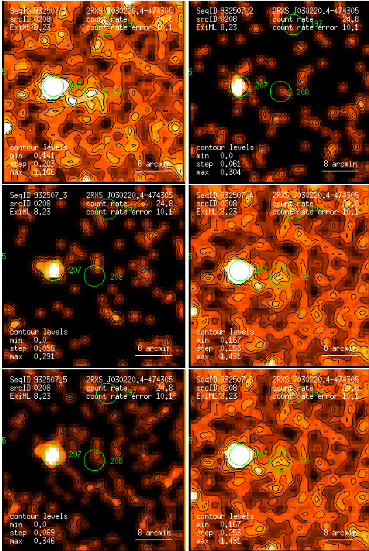
Figure 208: RASS 932507: detection 0208: band rate images, Gaussian filter: (1) PSPC channels 11 – 41, (2) 52 – 90, (3) 91 – 201, (4) 11 – 235, (5) 52 – 201, (6) 11 – 201. Broad band rates in counts/ks. Band rate contour levels in counts/ks/arcmin 2 .
