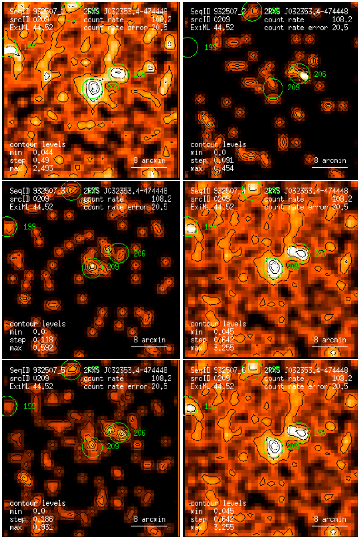
Figure 209: RASS 932507: detection 0209: band rate images, Gaussian filter: (1) PSPC channels 11 – 41, (2) 52 – 90, (3) 91 – 201, (4) 11 – 235, (5) 52 – 201, (6) 11 – 201. Broad band rates in counts/ks. Band rate contour levels in counts/ks/arcmin 2 .
